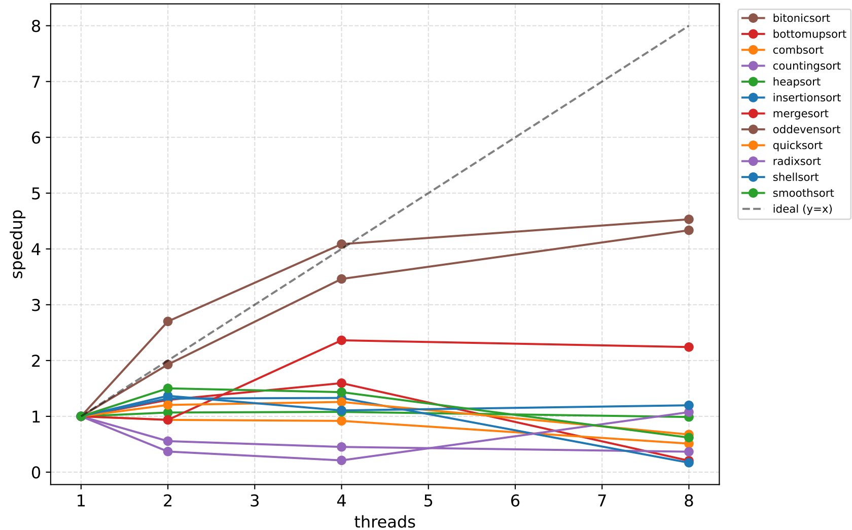
Speedup vs threads (N=100000) with ideal line
