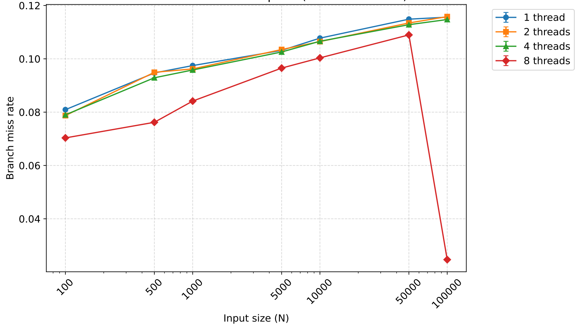
Branch miss rate - bottomupsort (mean +- 95% CI)
