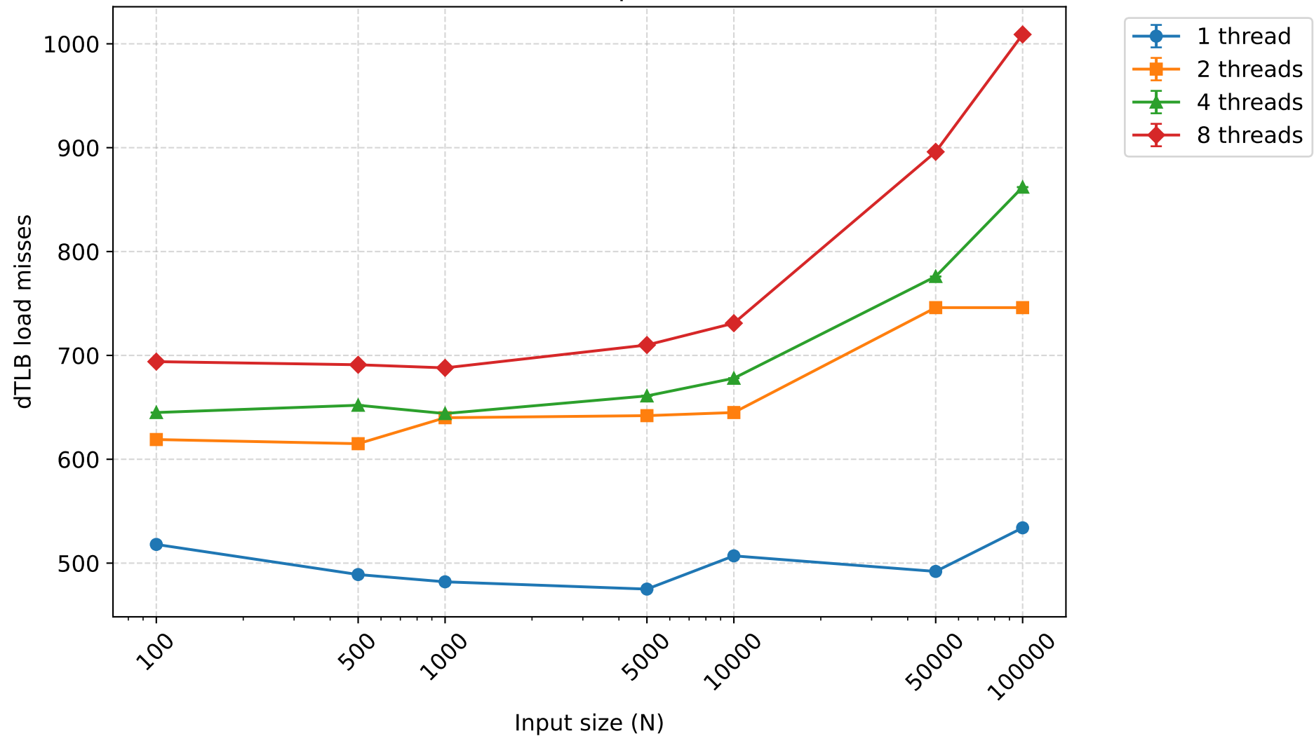
dTLB load misses - bottomupsort (mean \pm 95% CI)
