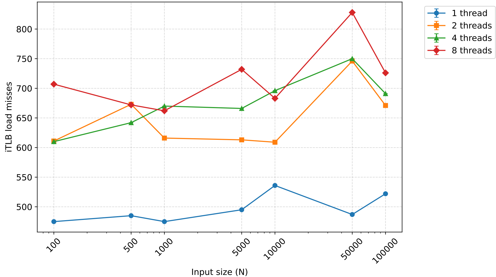
iTLB load misses - bottomupsort (mean \pm 95% CI)
