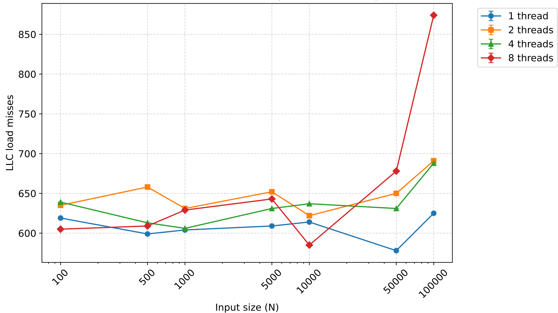
LLC load misses - combort (mean \pm 95% CI)
