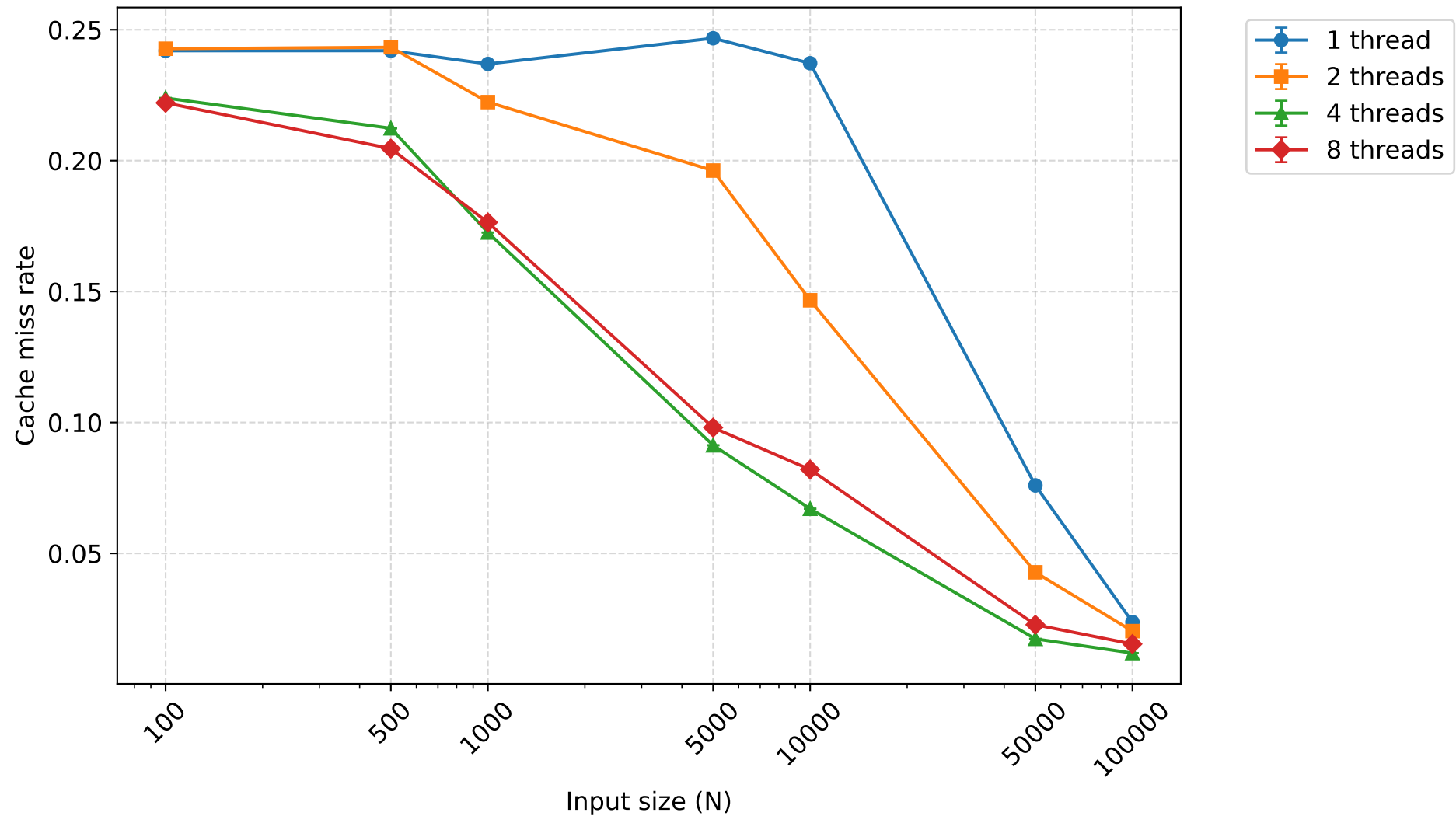
Cache miss rate - combort (mean \pm 95% CI)
