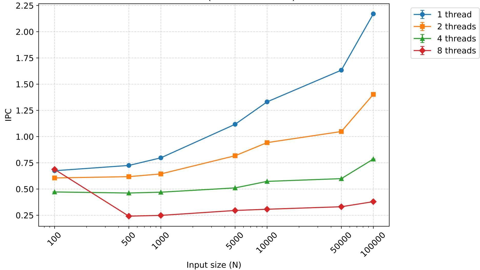
IPC - combSORT (mean \pm 95% CI)
