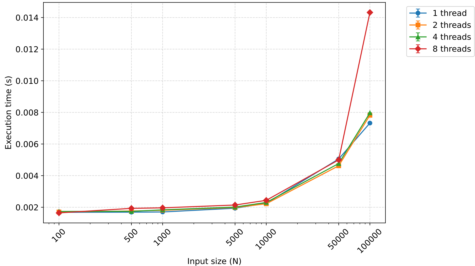
Execution time (s) - combSort (mean \pm 95% CI)
