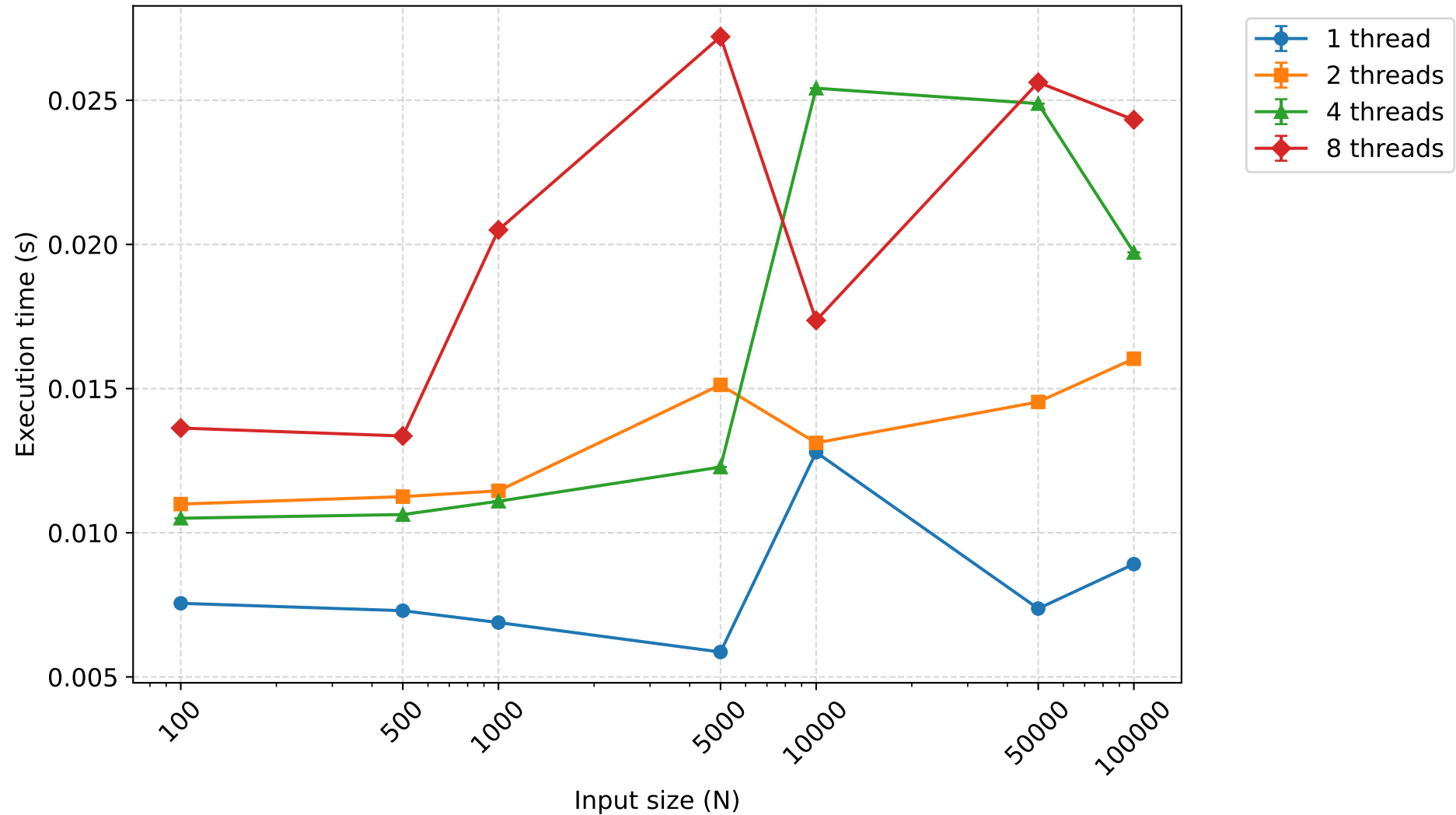
Execution time (s) - counting sort (mean \pm 95% CI)
