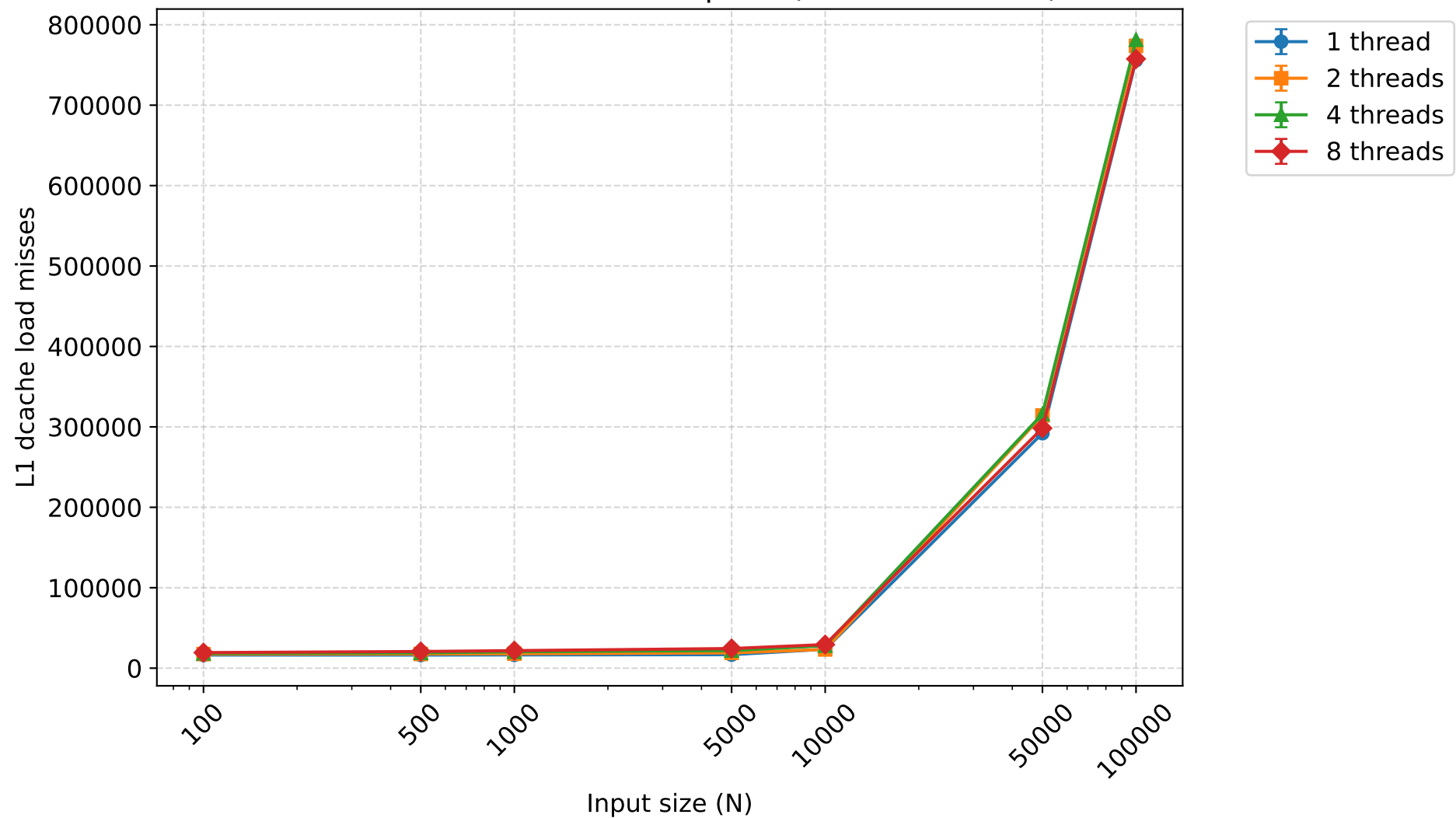
L1 dcache load misses - heapsort (mean \pm 95% CI)
