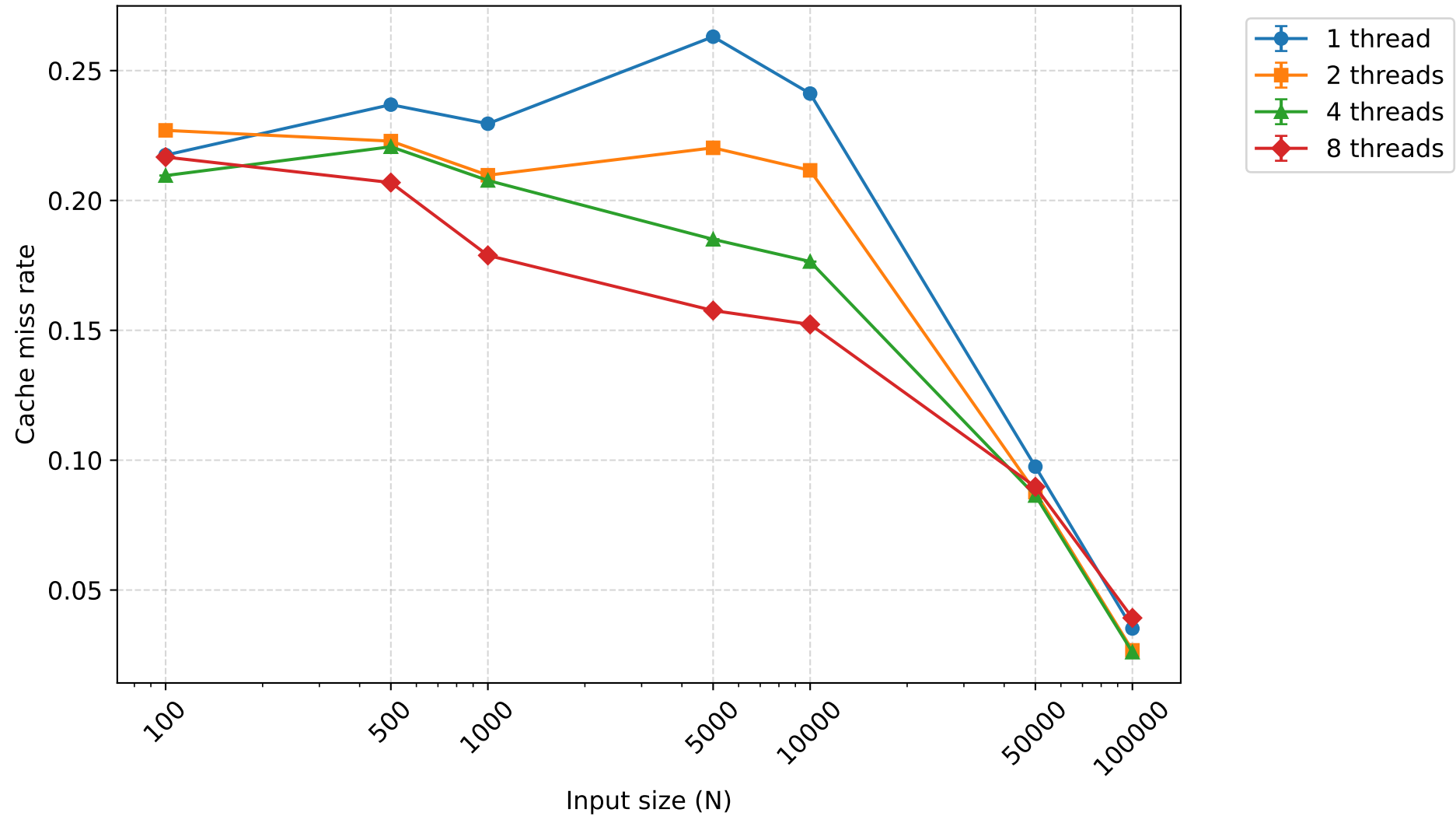
Cache miss rate - heapsort (mean \pm 95% CI)
