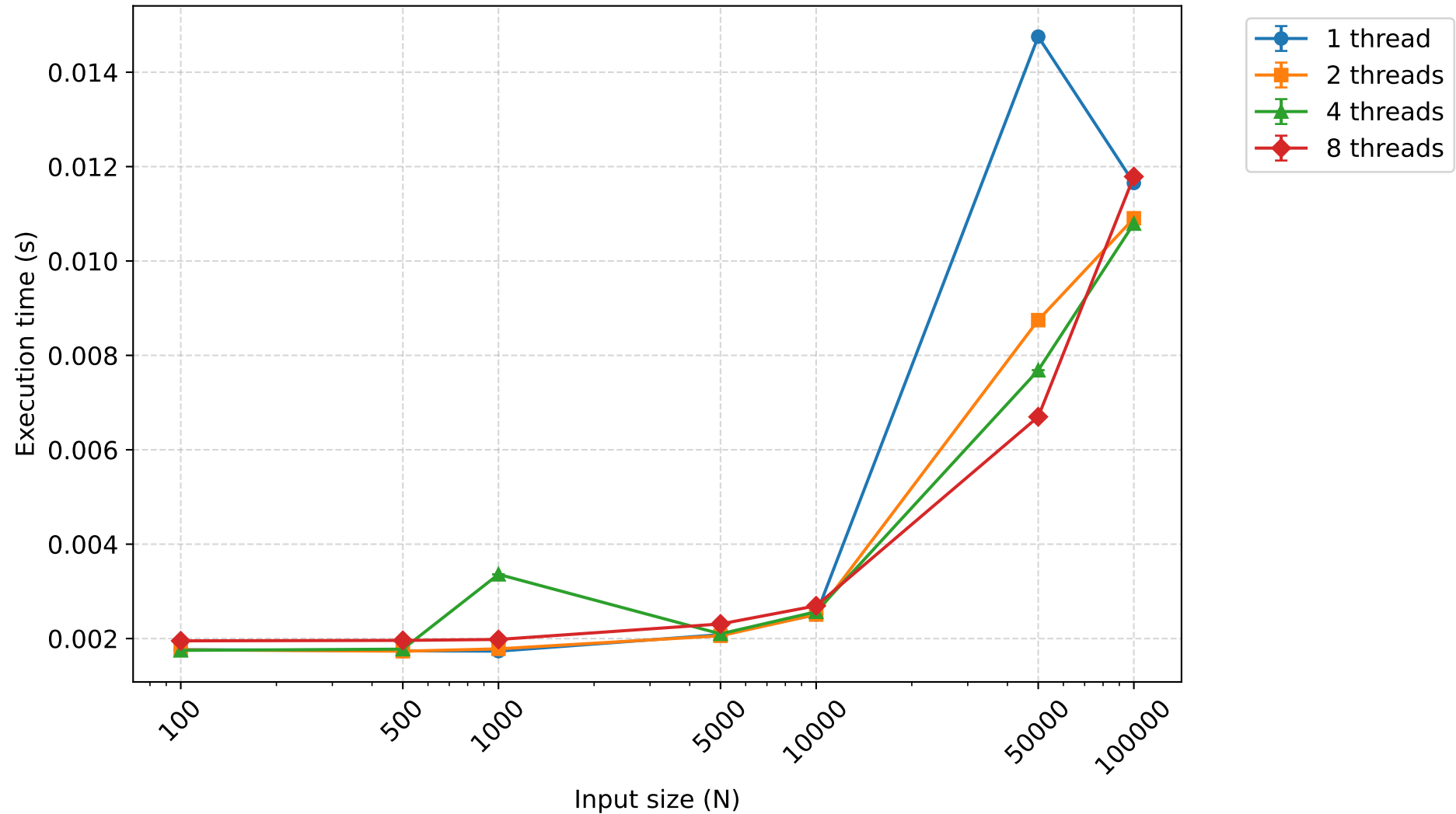
Execution time (s) - heapsort (mean \pm 95% CI)
