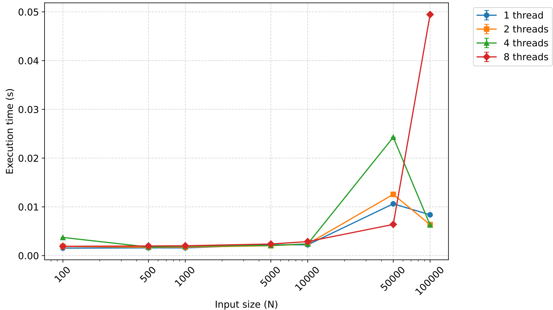
Execution time (s) - insertionsort (mean \pm 95% CI)
