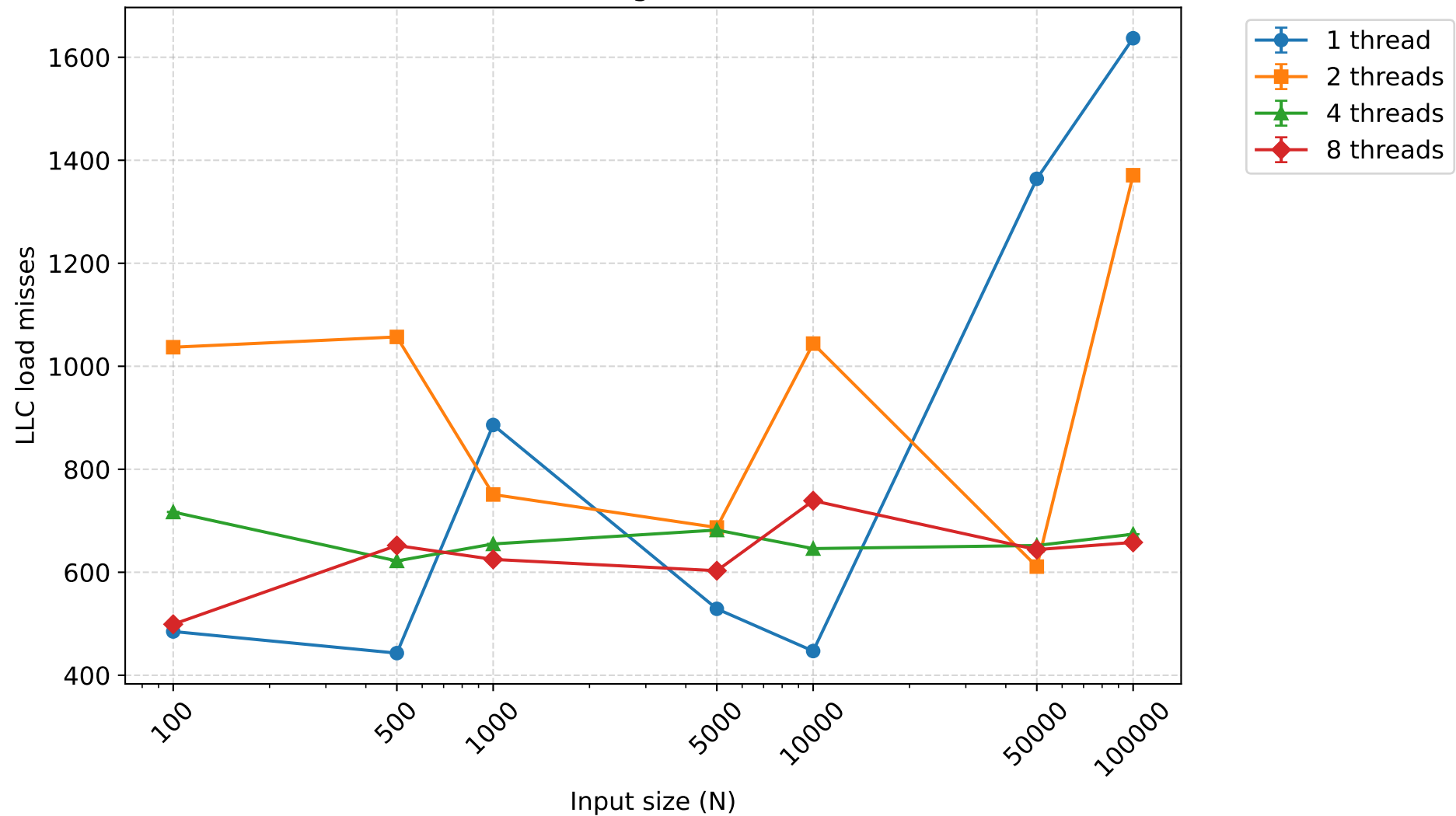
LLC load misses - mergesort (mean \pm 95% CI)
