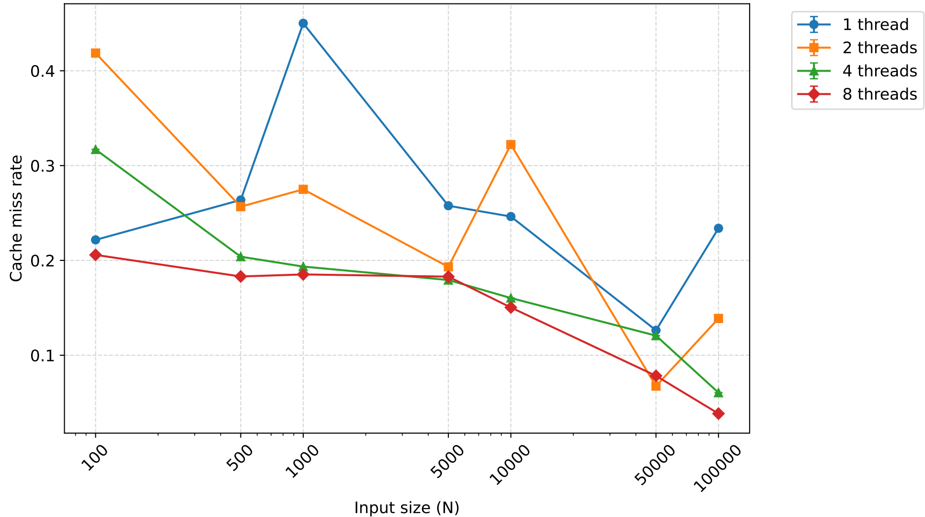
Cache miss rate - mergesort (mean \pm 95% CI)
