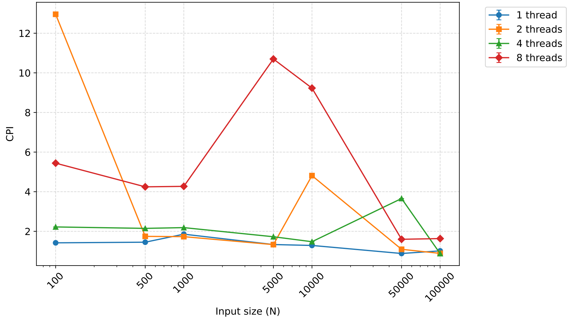
CPI - mergesort (mean \pm 95% CI)
