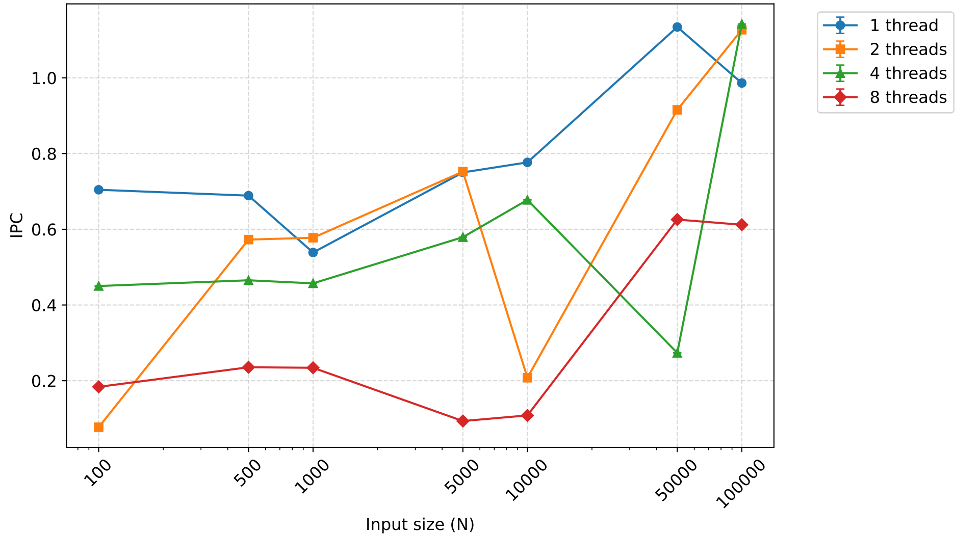
IPC - mergesort (mean \pm 95% CI)
