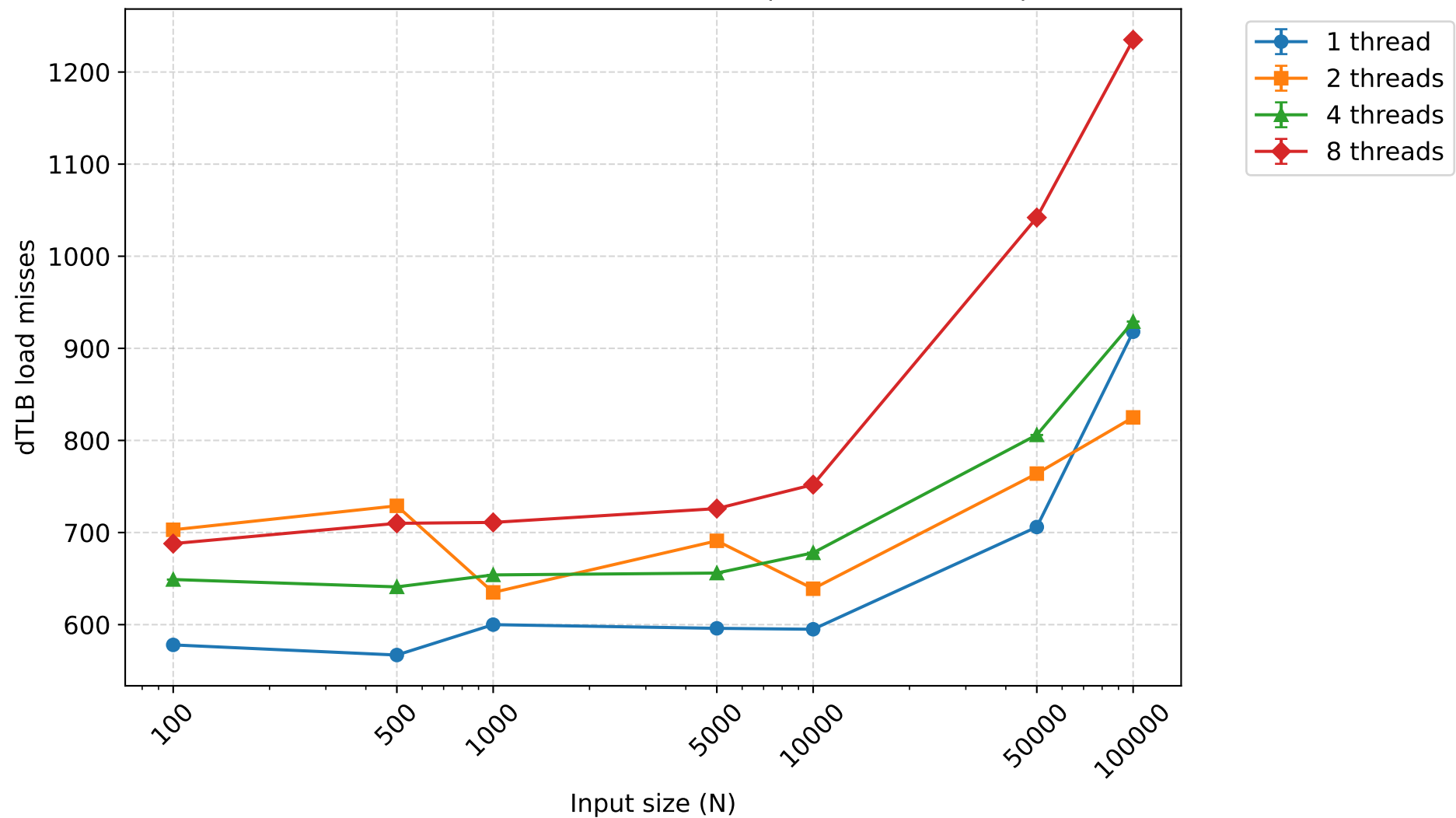
dTLB load misses - oddevensort (mean \pm 95% CI)
