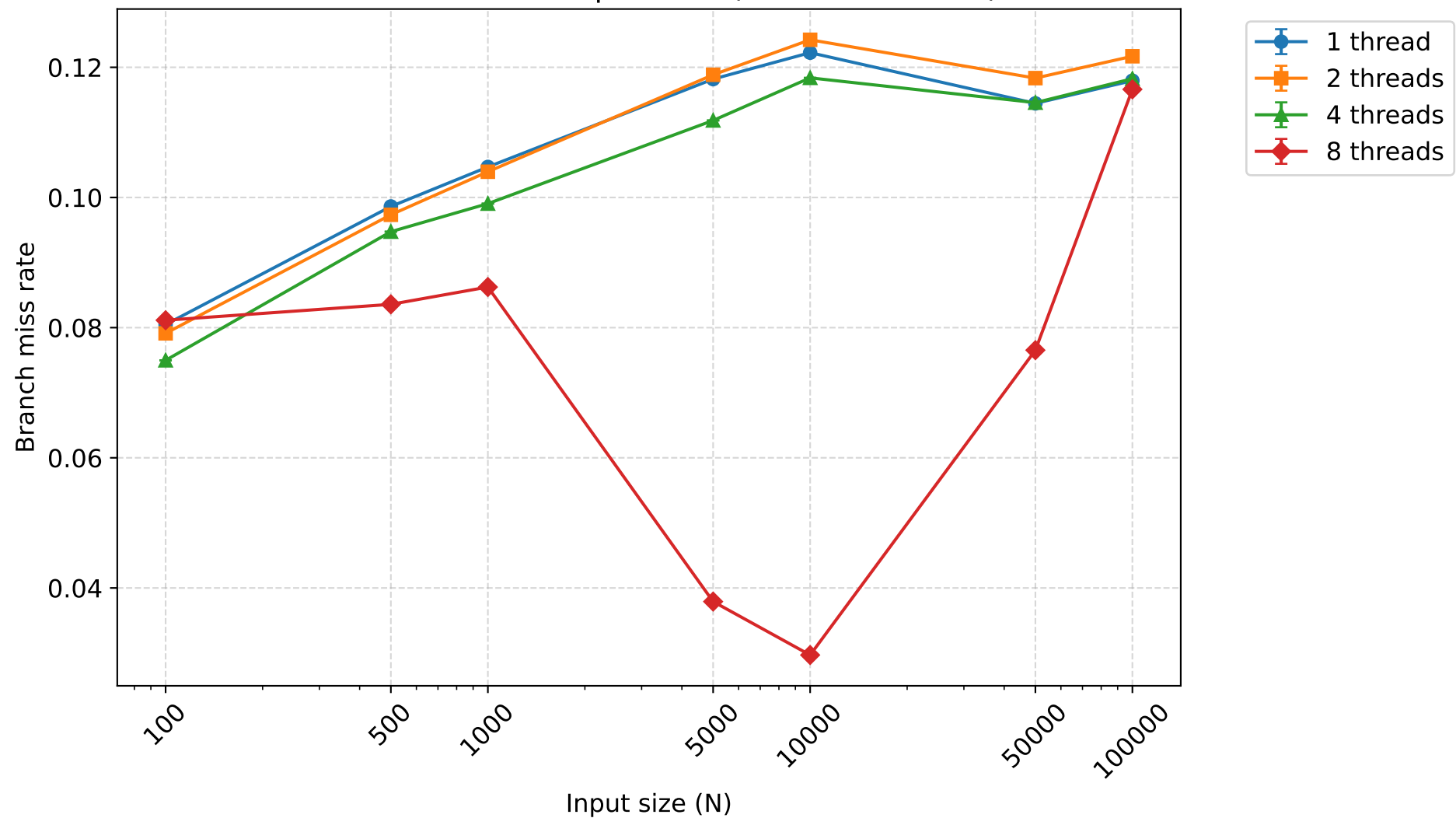
Branch miss rate - quicksort (mean \pm 95% CI)
