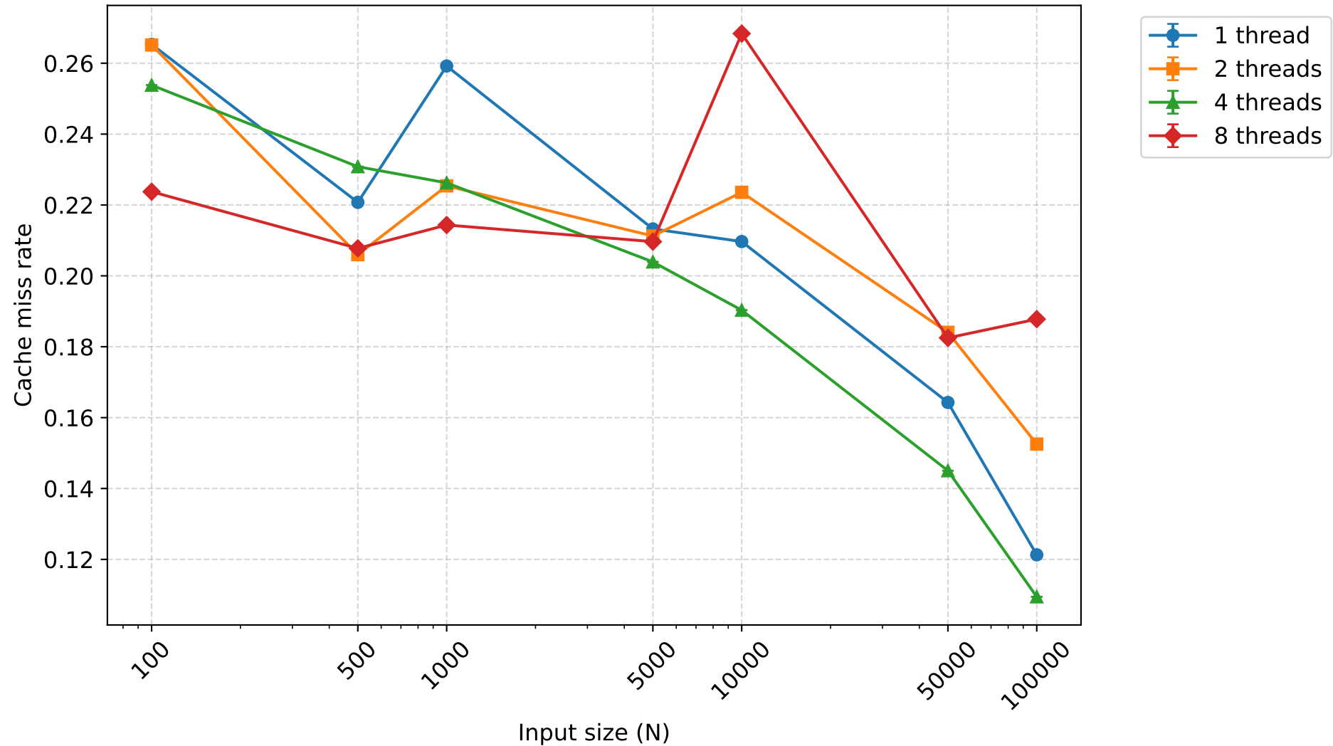
Cache miss rate - quicksort (mean \pm 95% CI)
