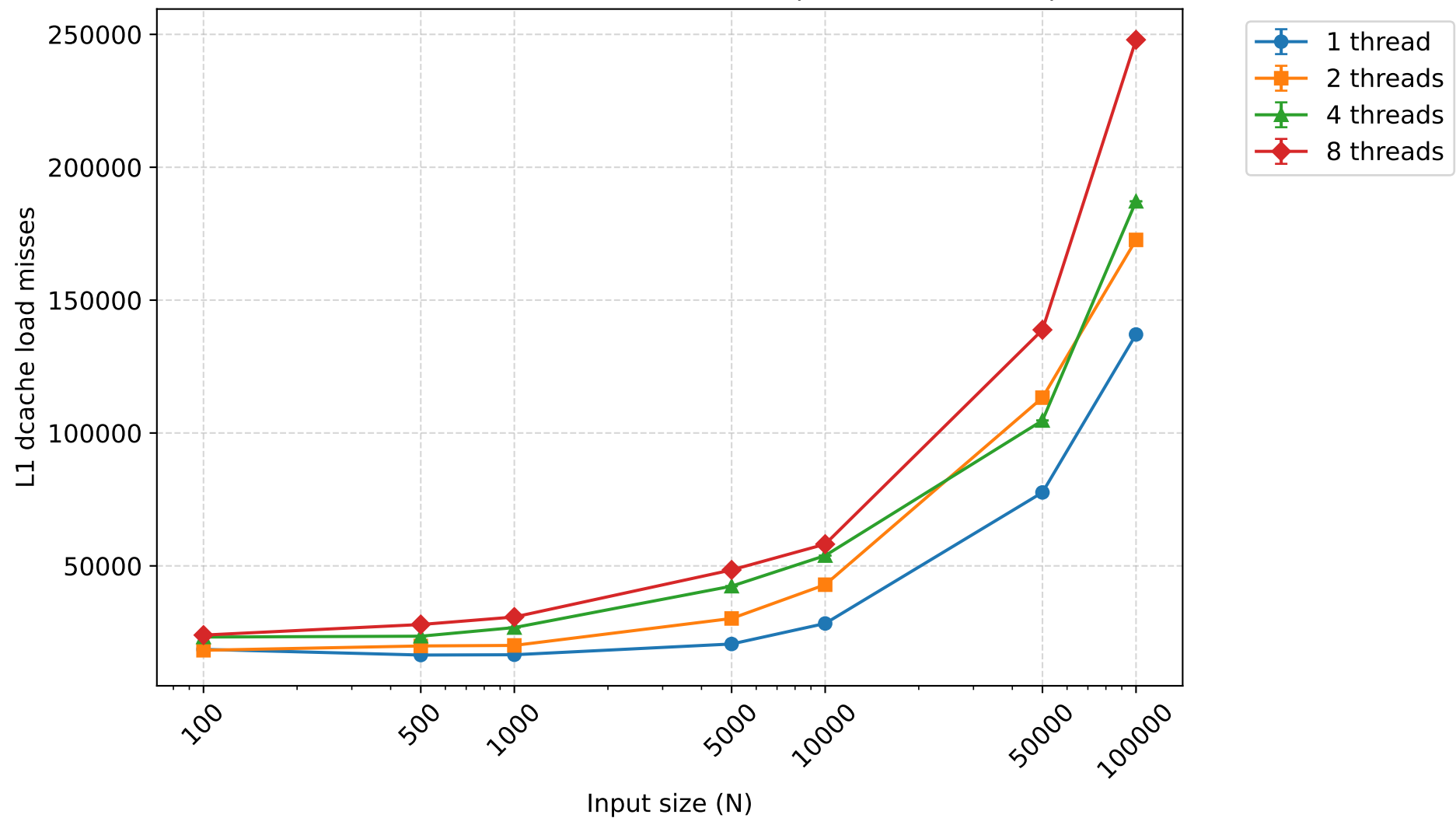
L1 dcache load misses - radixsort (mean \pm 95% CI)
