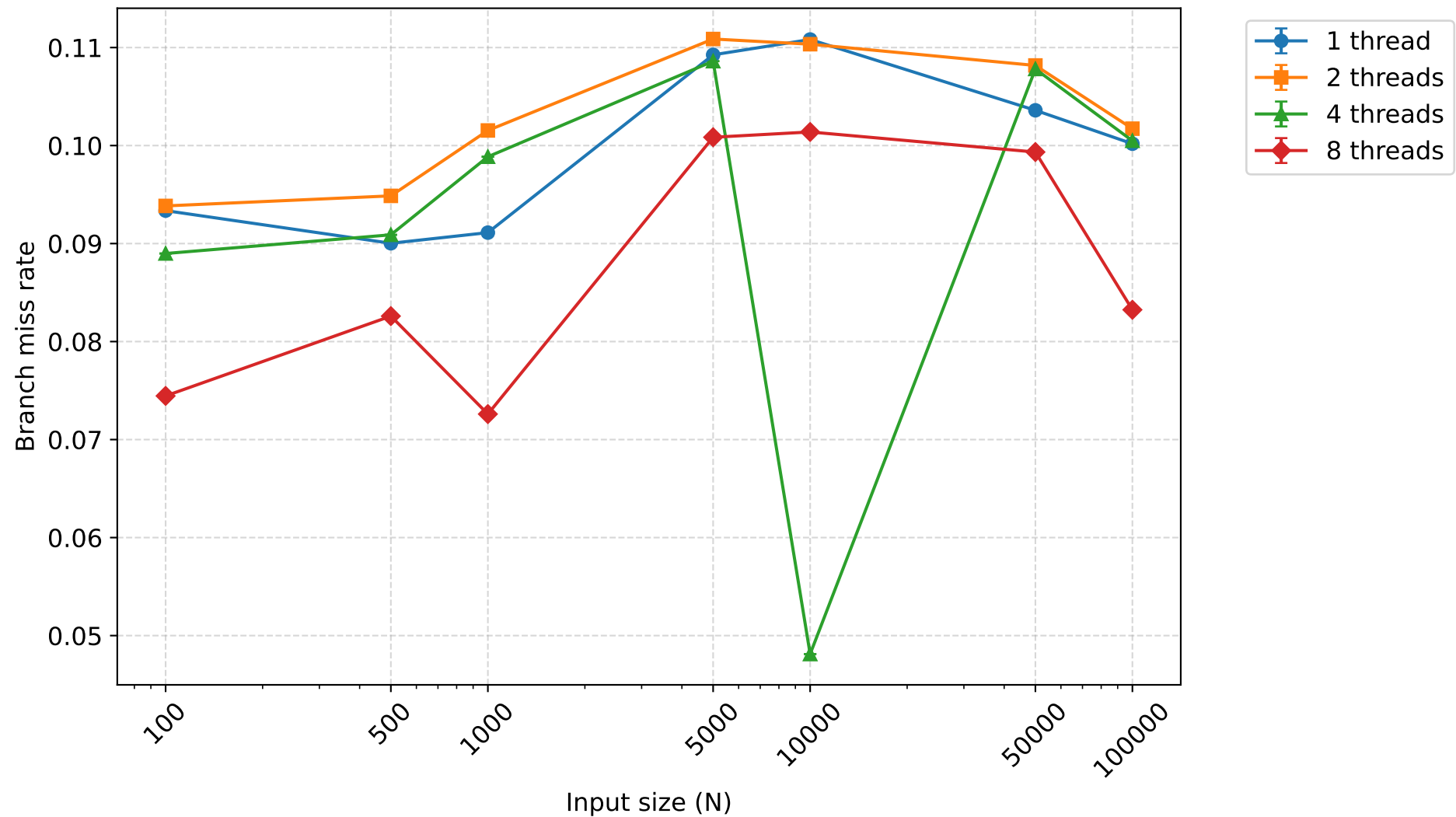
Branch miss rate - shellsort (mean \pm 95% CI)
