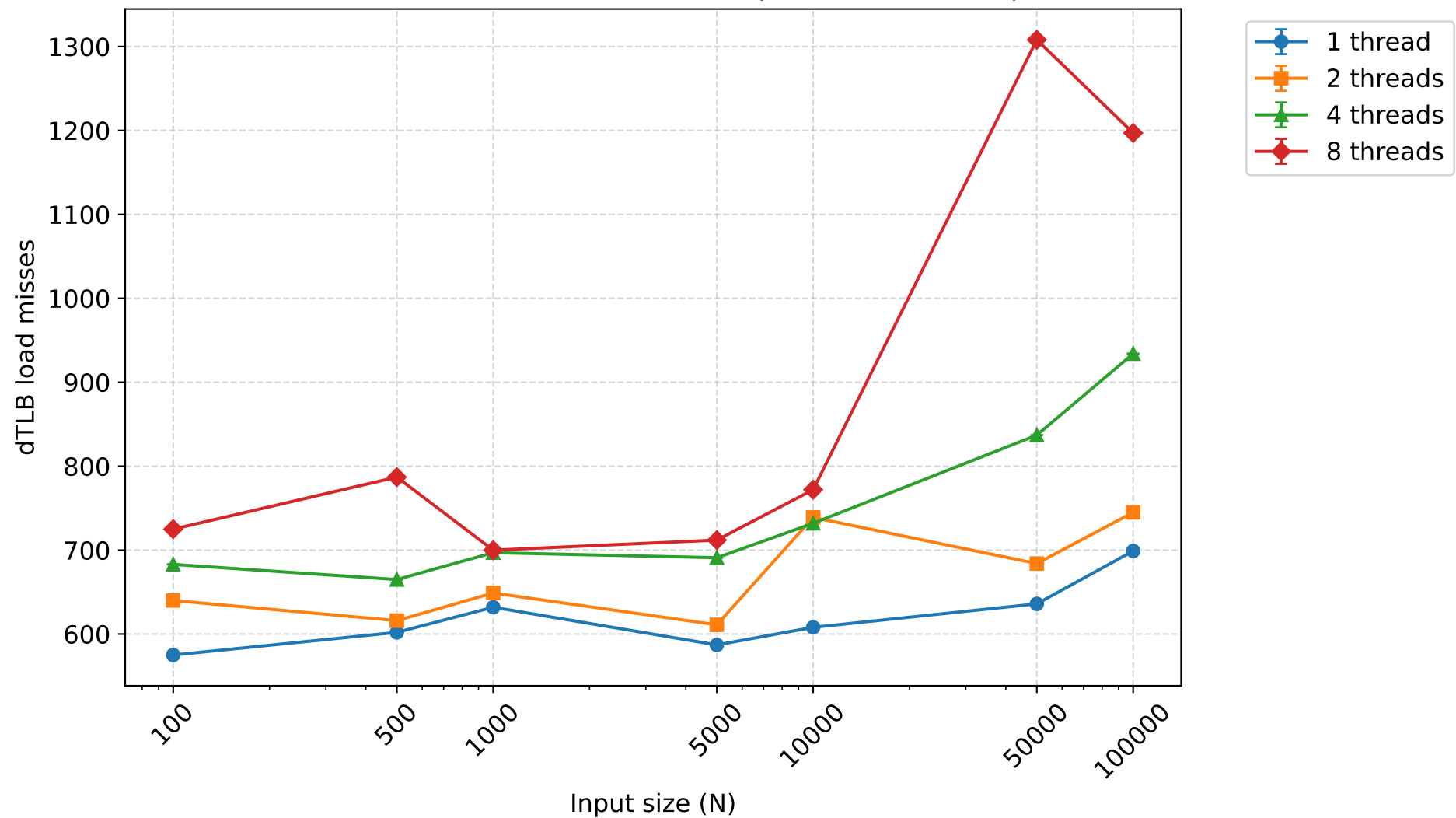
dTLB load misses - smoothsort (mean \pm 95% CI)
