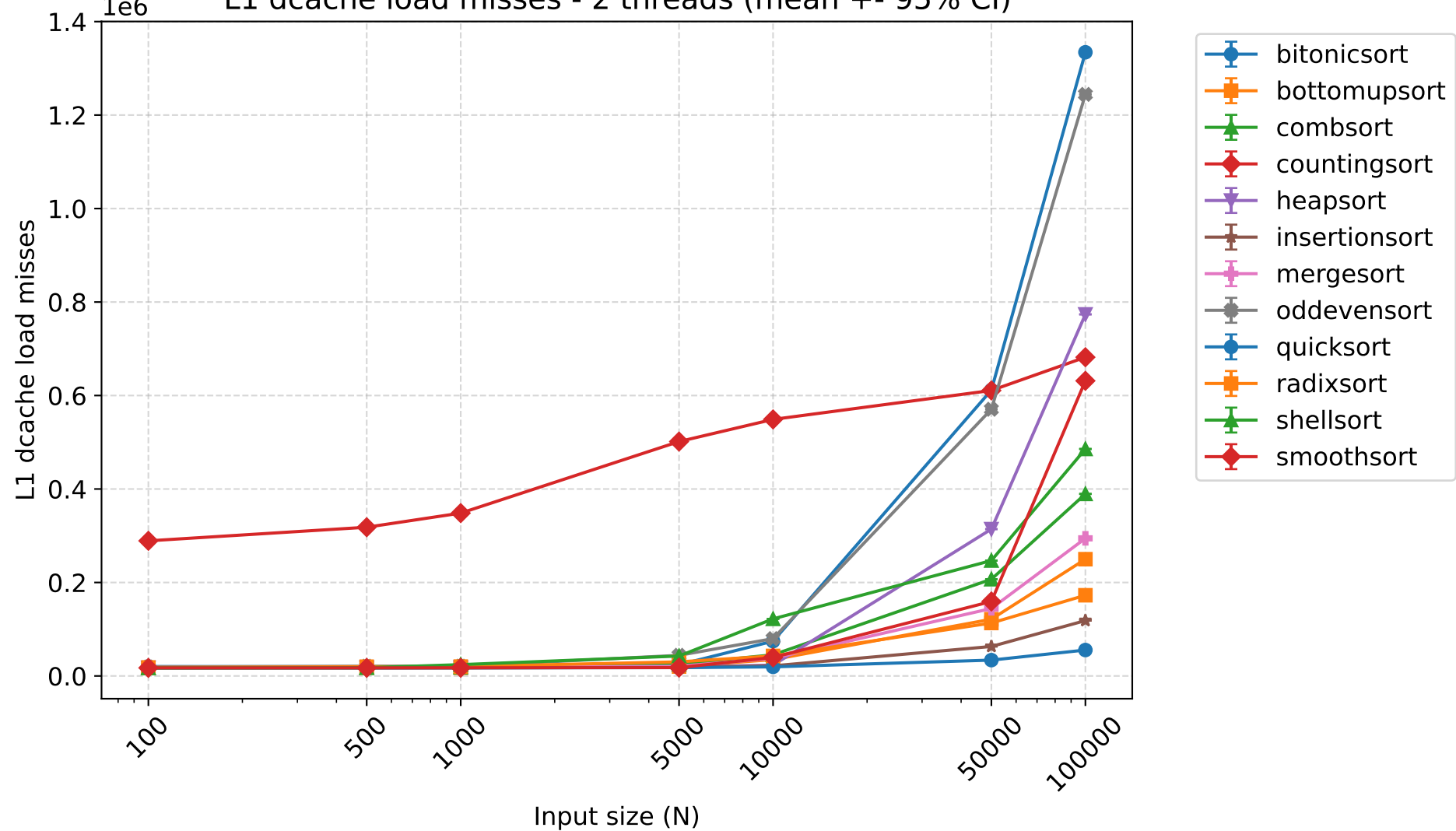
L1 dcache load misses - 2 threads (mean \pm 95% CI)
