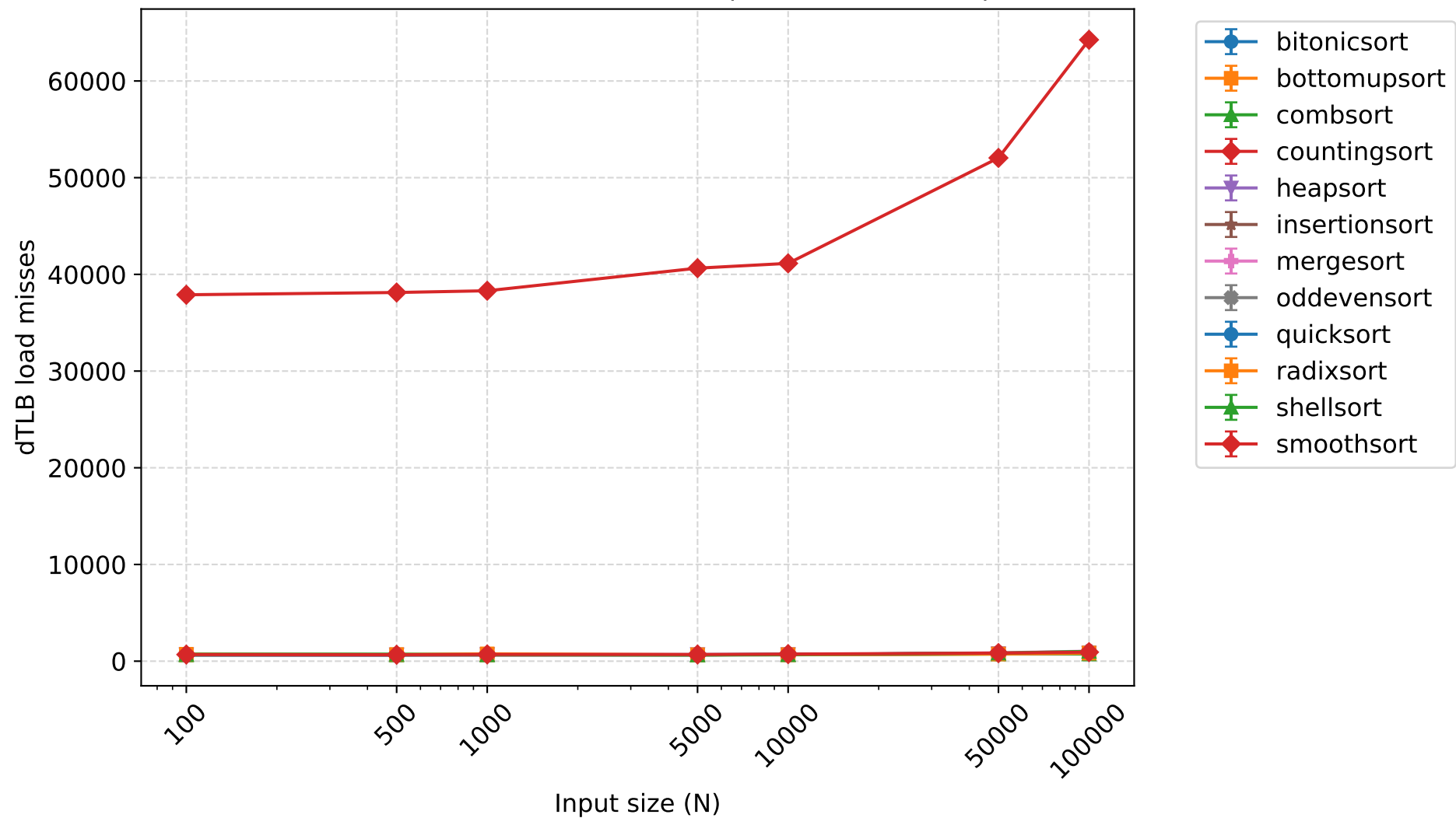
dTLB load misses - 4 threads (mean +- 95% CI)
