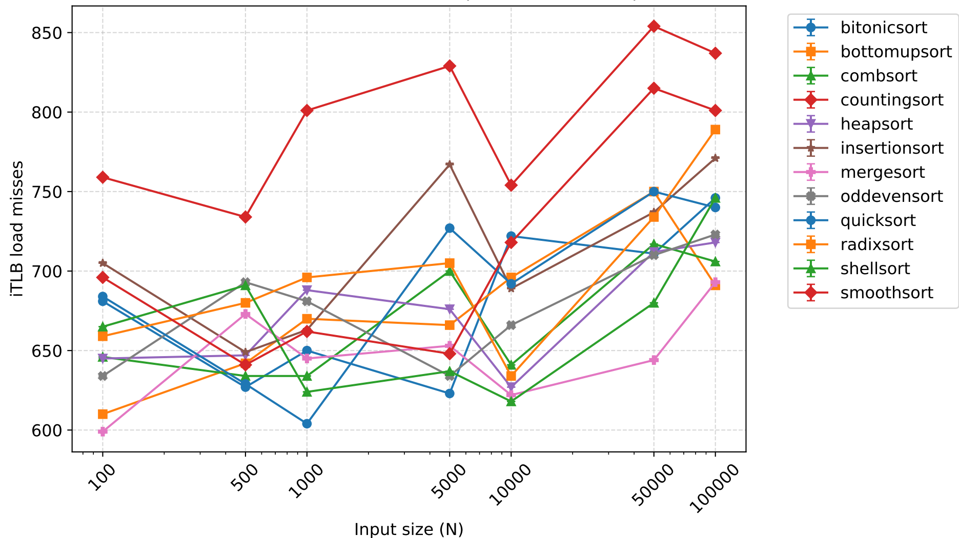
iTLB load misses - 4 threads (mean \pm 95% CI)
