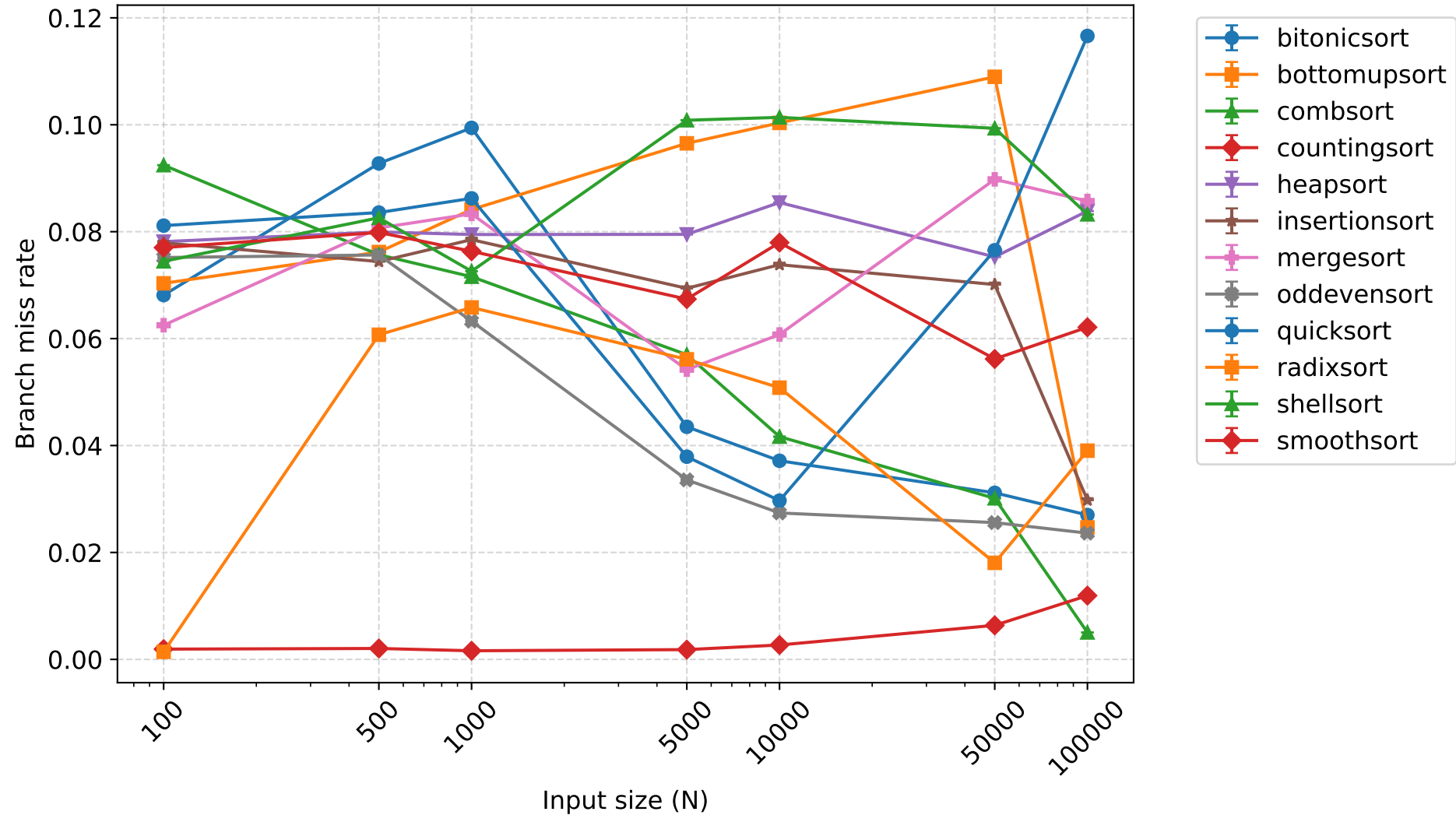
Branch miss rate - 8 threads (mean \pm 95% CI)
