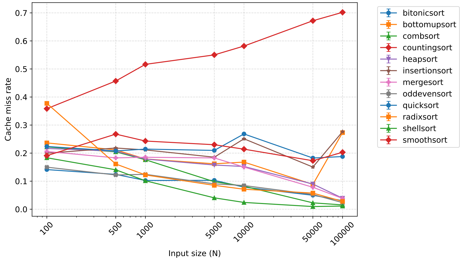
Cache miss rate - 8 threads (mean \pm 95% CI)
