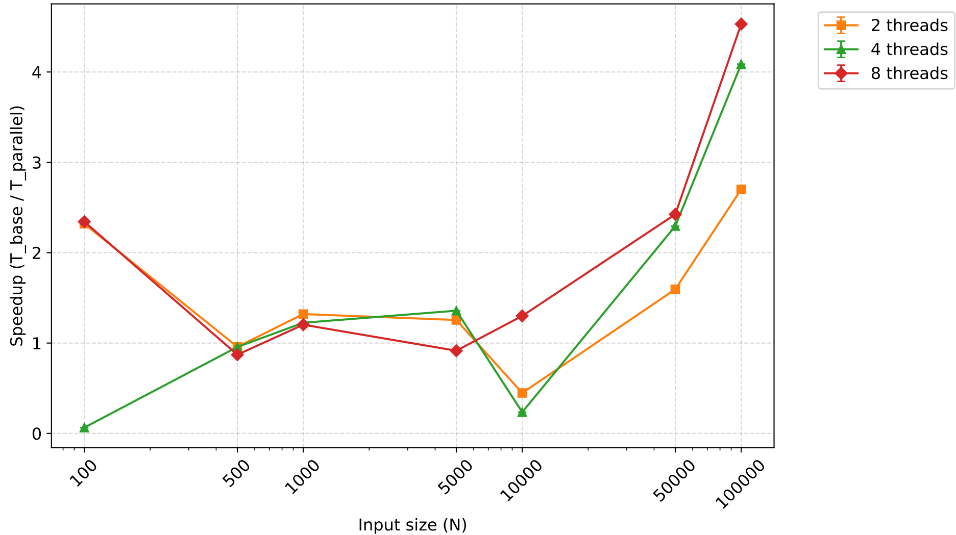
Speedup - bitonicsort (mean \pm 95% CI)
