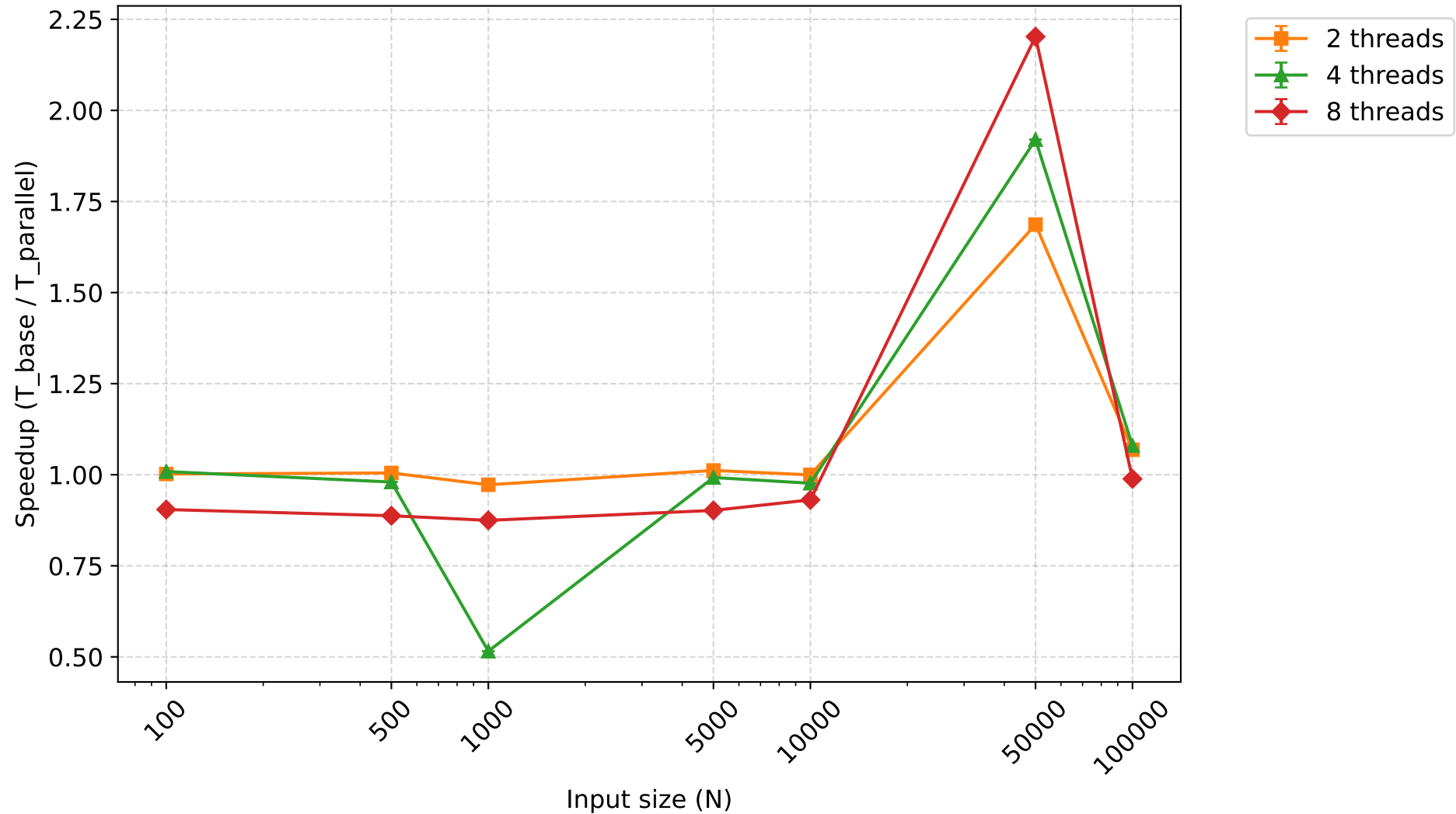
Speedup - heapsort (mean \pm 95% CI)
