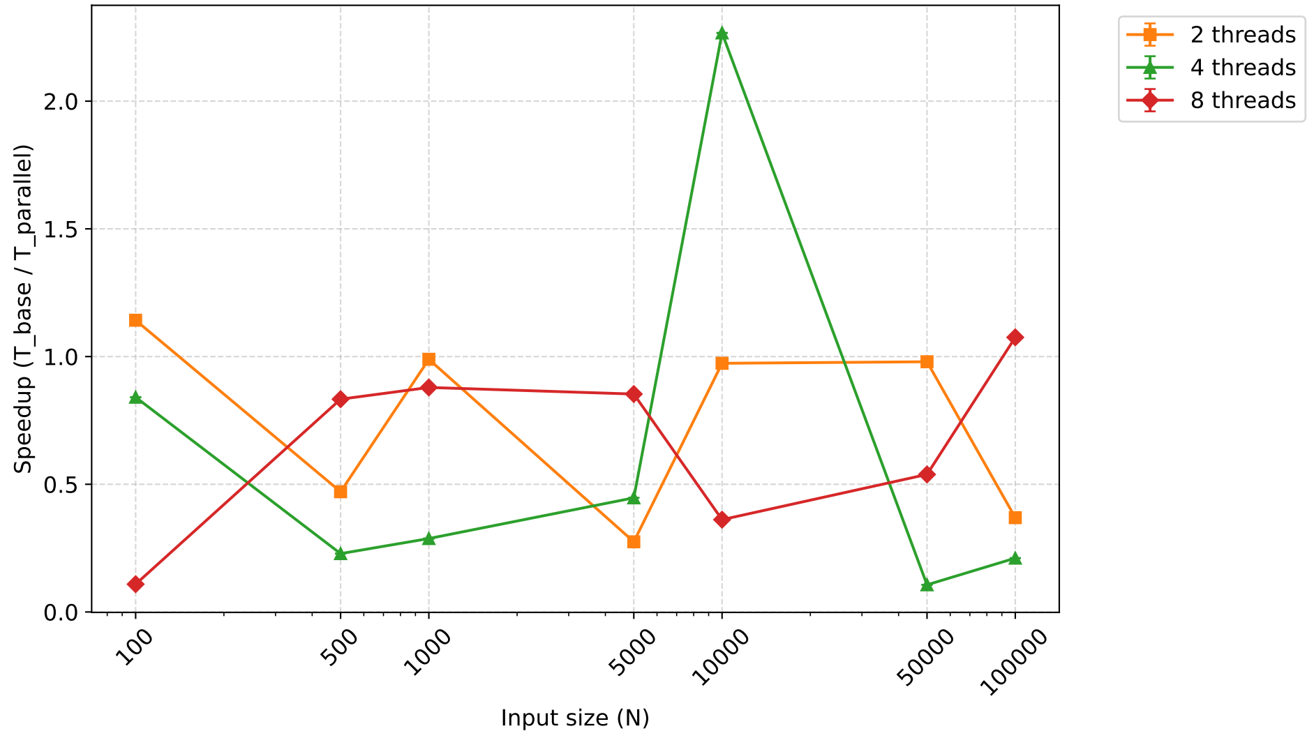
Speedup - radixsort (mean +- 95% CI)
