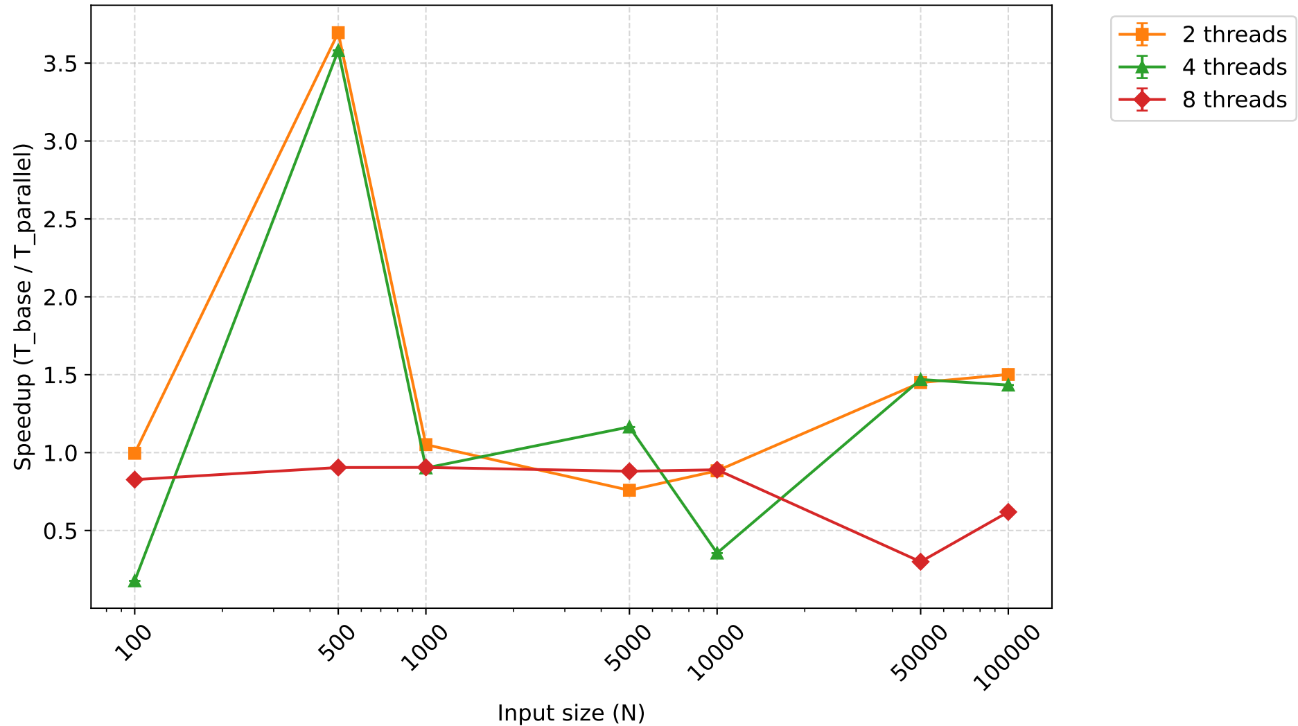
Speedup - smoothsort (mean \pm 95% CI)
