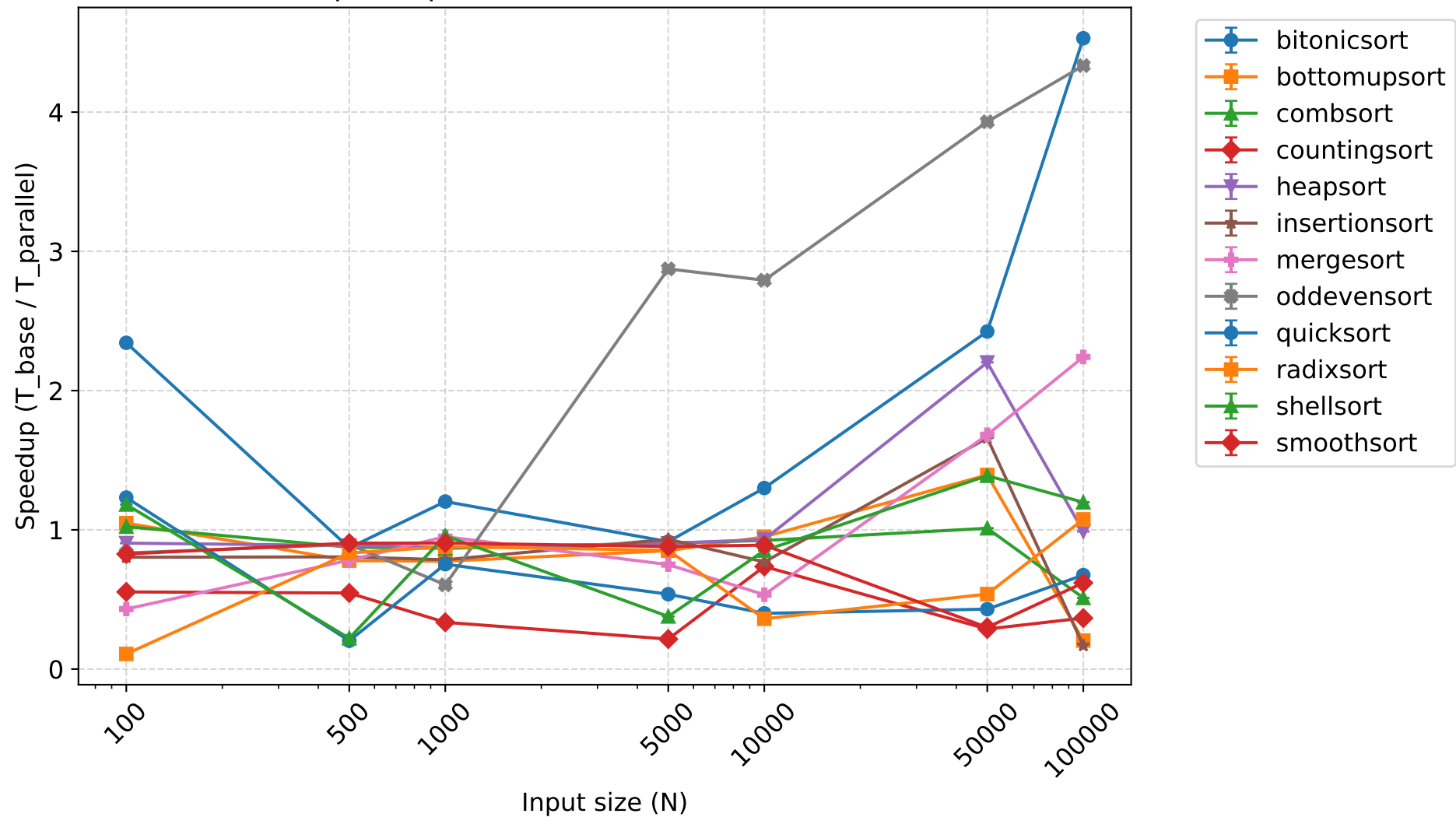
Speedup - 8 threads (mean \pm 95% CI)
