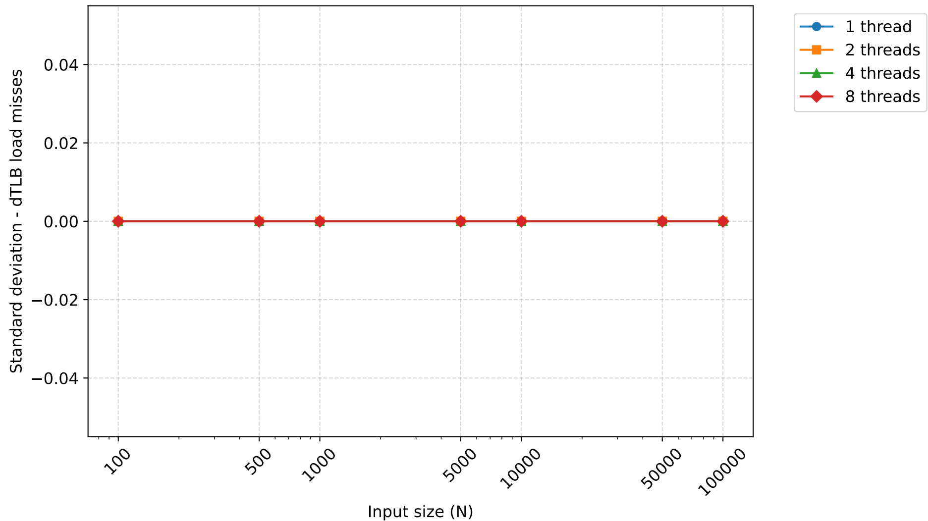
Standard deviation of dTLB load misses - bitonicsort
