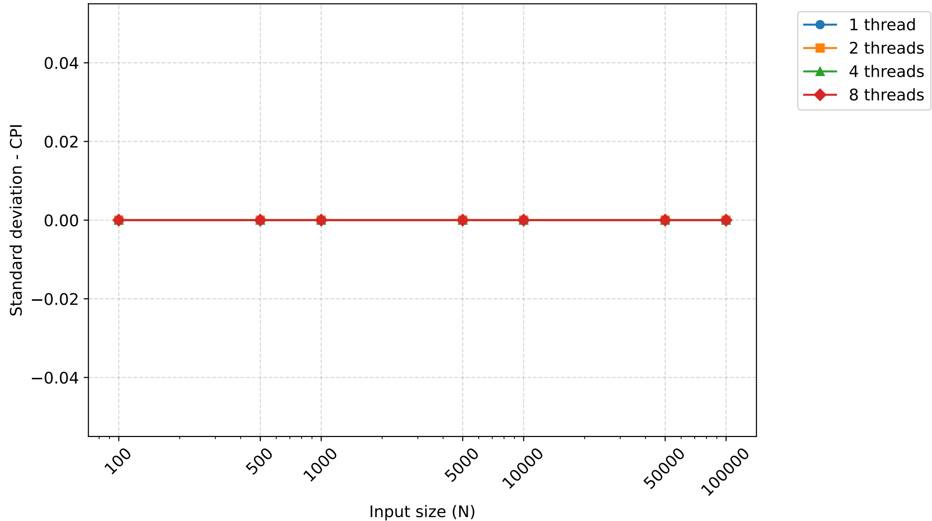
Standard deviation of CPI - counting sort
