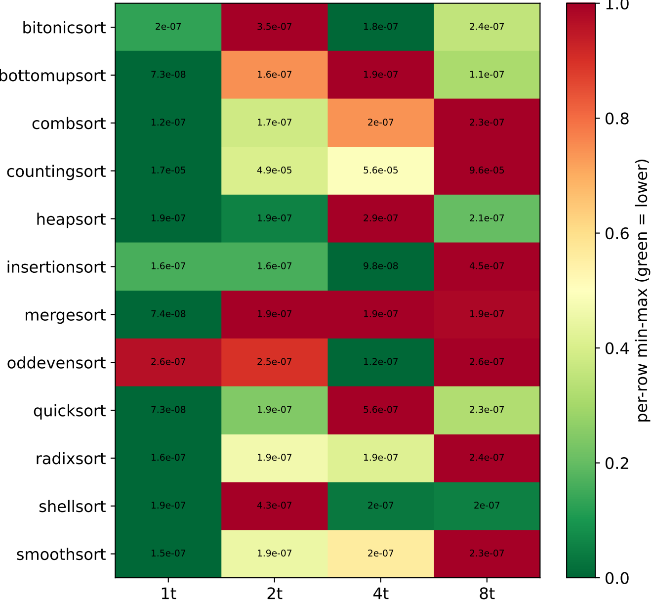
ED 2 P (J·s 2 ) by algorithm × threads (N=1000) — green = best per row
