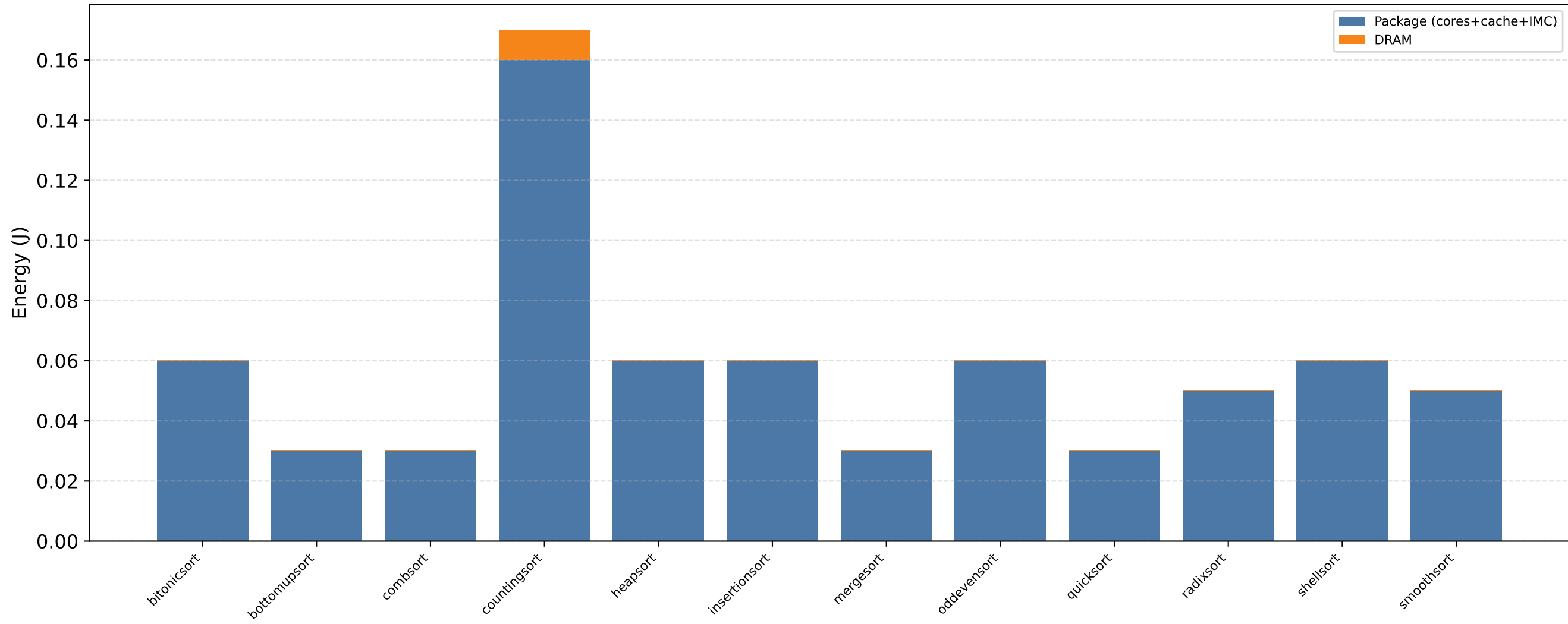
Energy breakdown: package vs DRAM (N=1000, serial)
