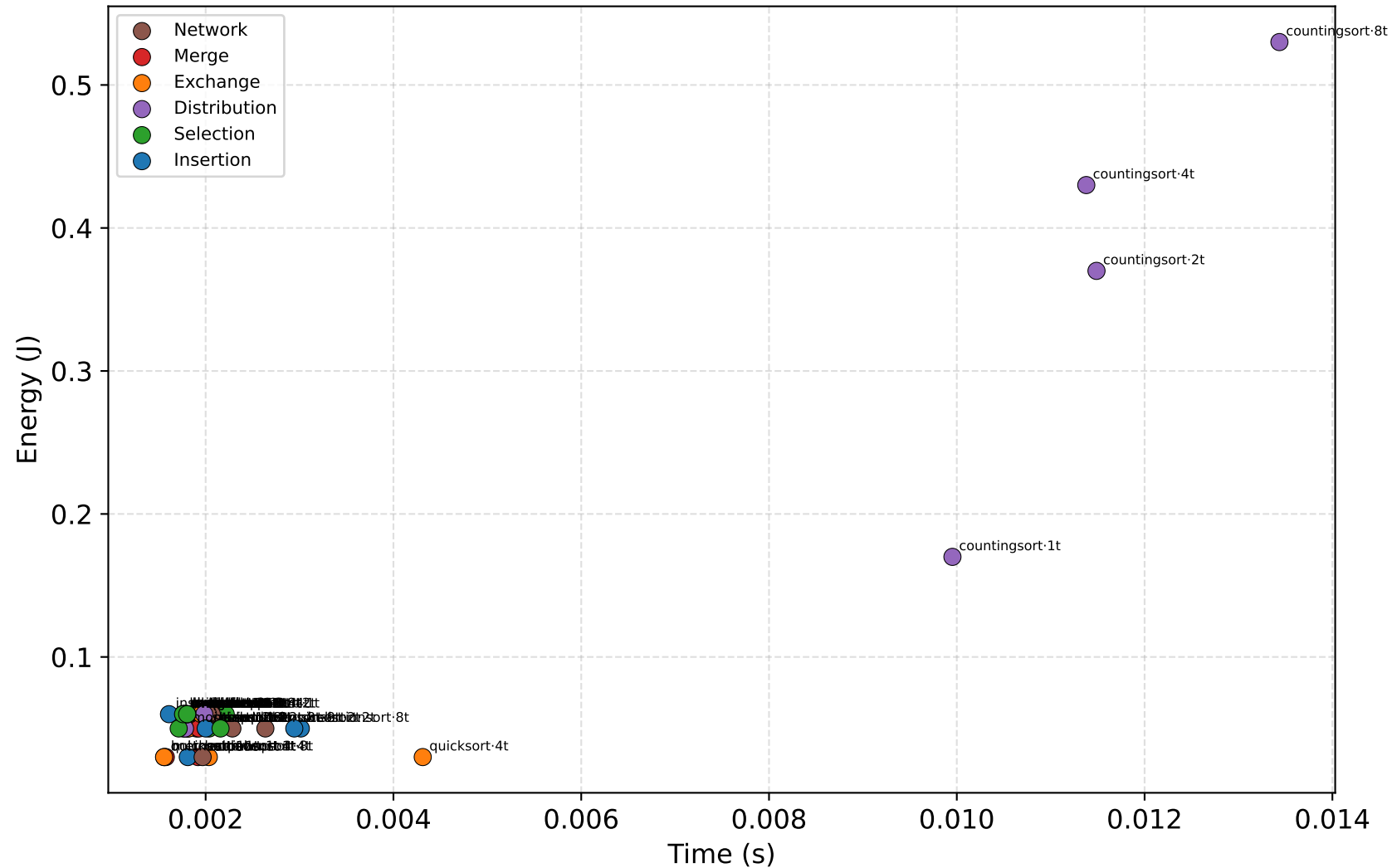
Energy-time trade-off (N=1000, all thread counts)
