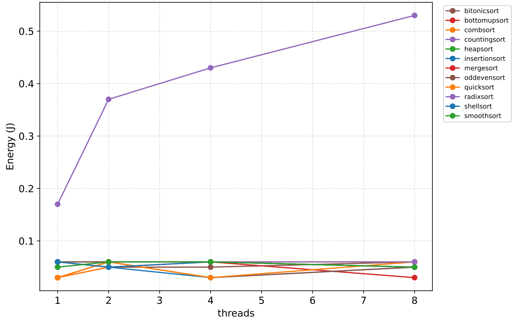
Total energy vs threads (N=1000) — does not drop like time
