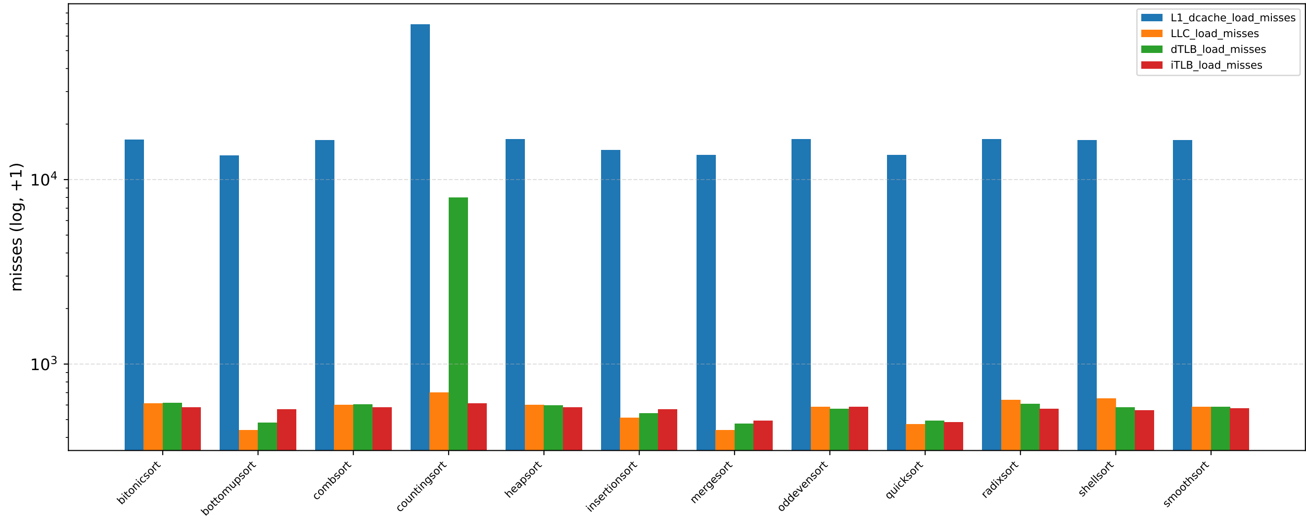
Memory hierarchy pressure (N=1000, serial)
