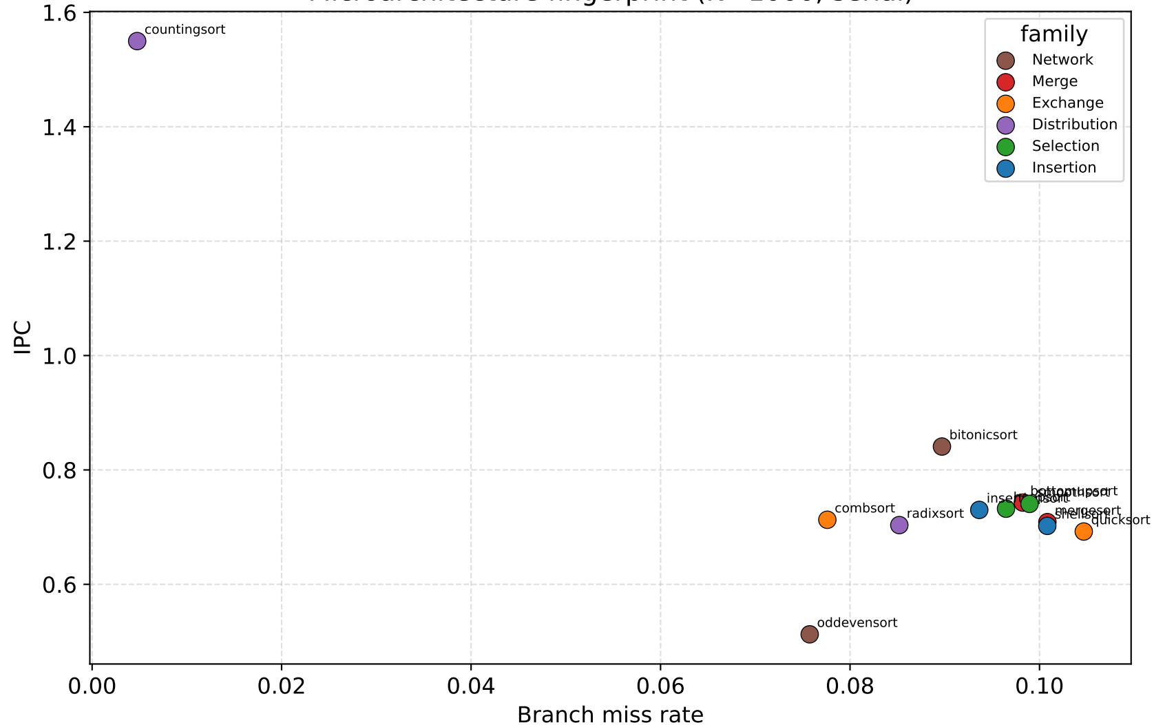
Microarchitecture fingerprint (N=1000, serial)
