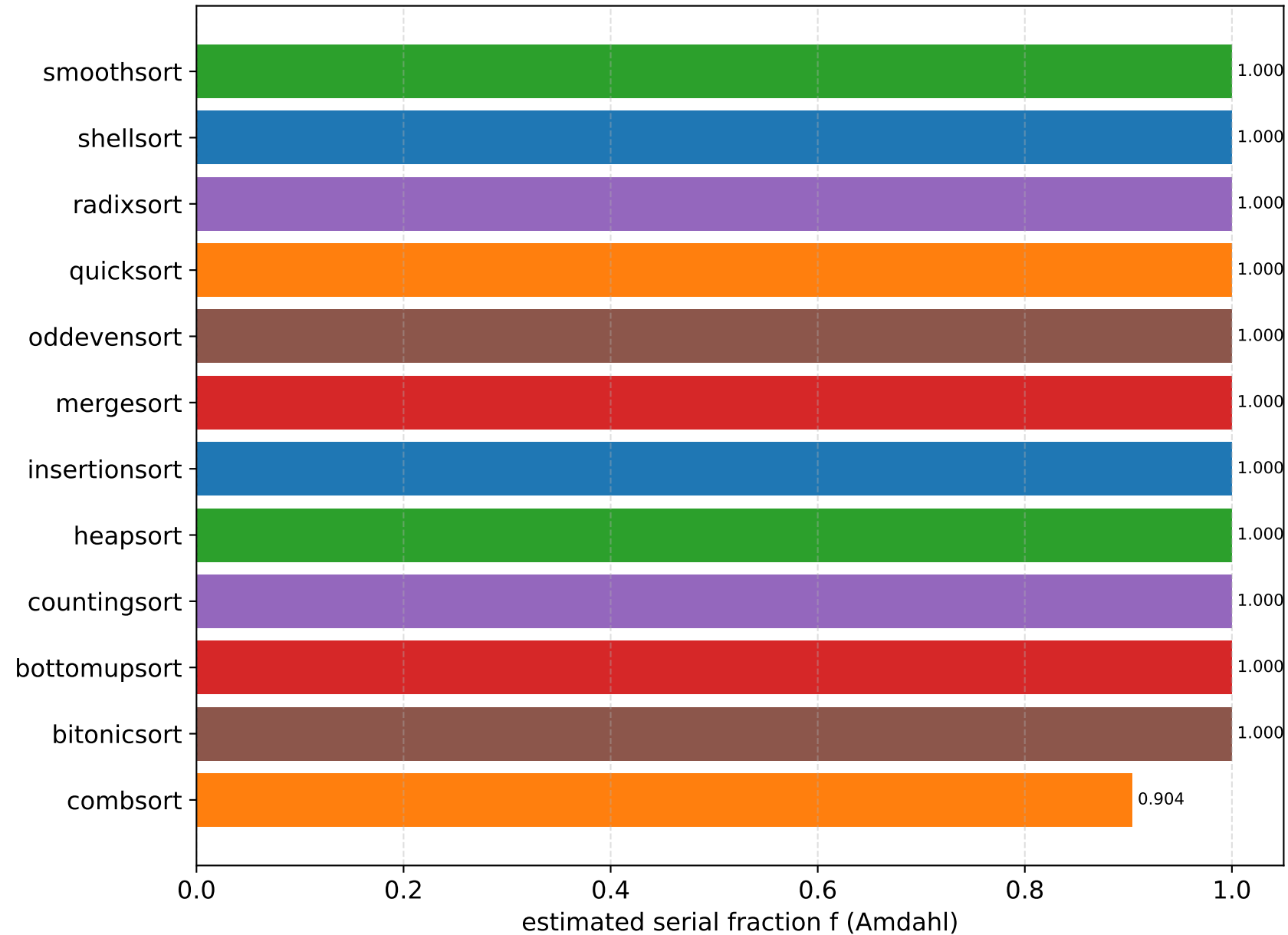
Serial fraction per algorithm (N=1000) — lower f scales better
