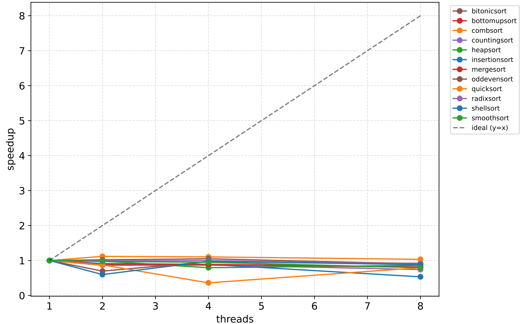
Speedup vs threads (N=1000) with ideal line
