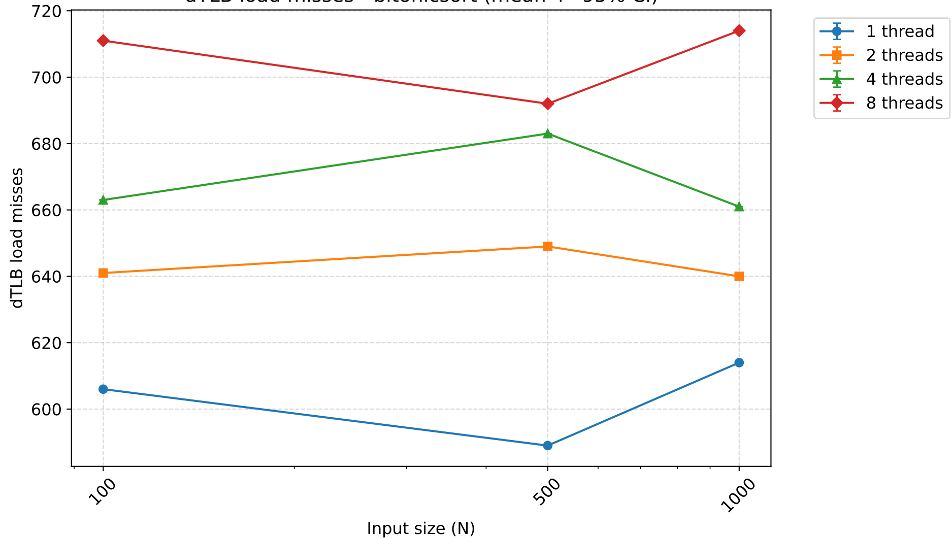
dTLB load misses - bitonicsort (mean \pm 95% CI)
