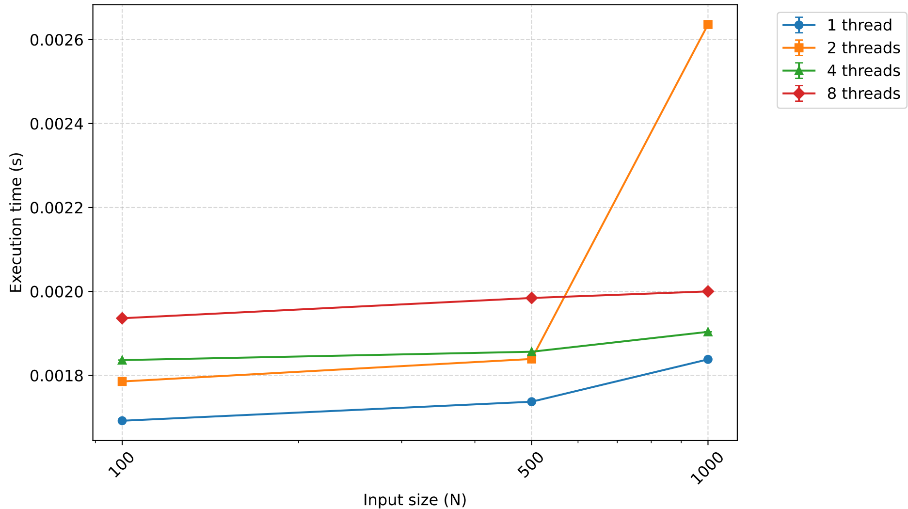
Execution time (s) - bitonicsort (mean \pm 95% CI)
