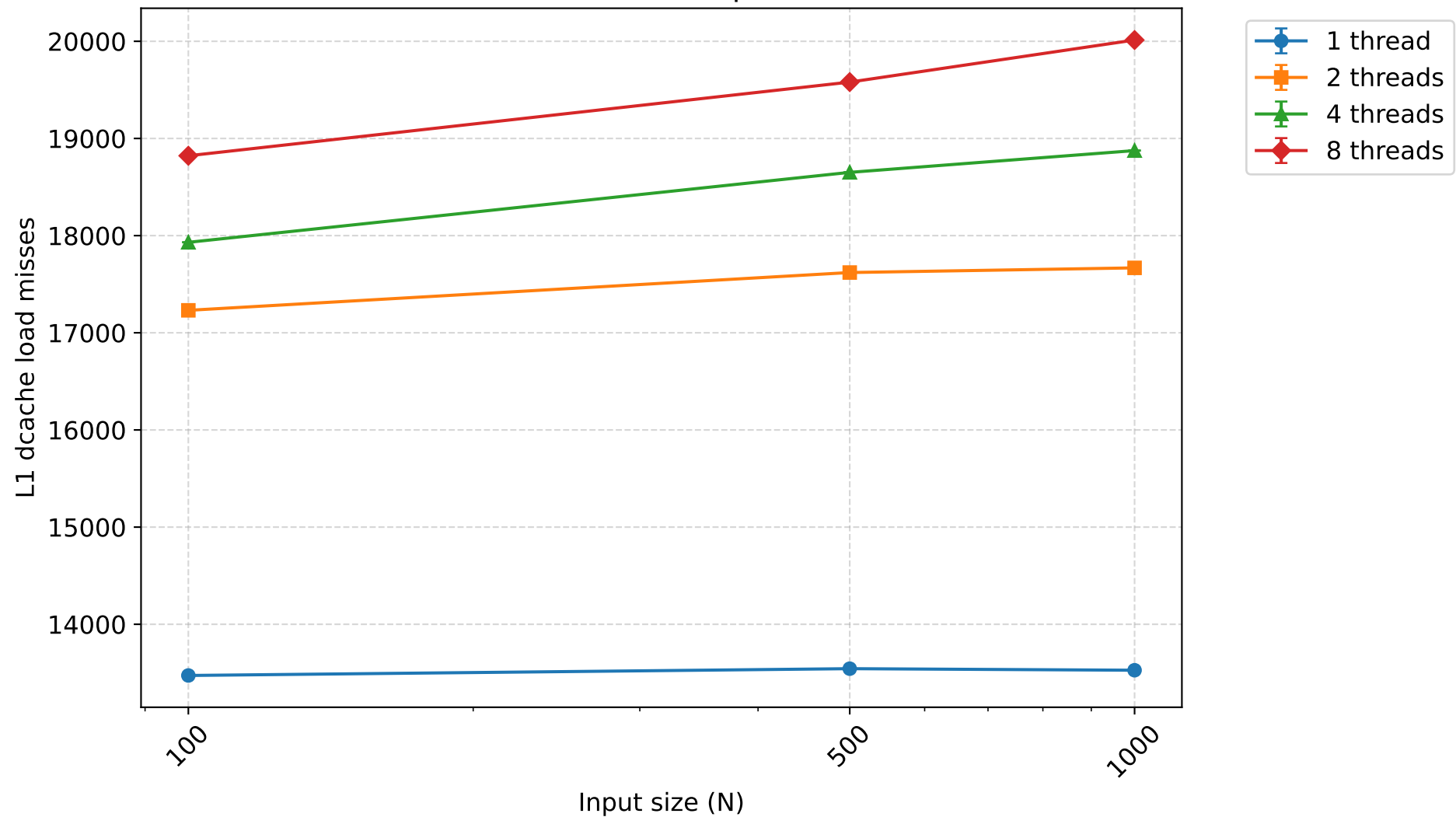
L1 dcache load misses - bottomupsort (mean \pm 95% CI)
