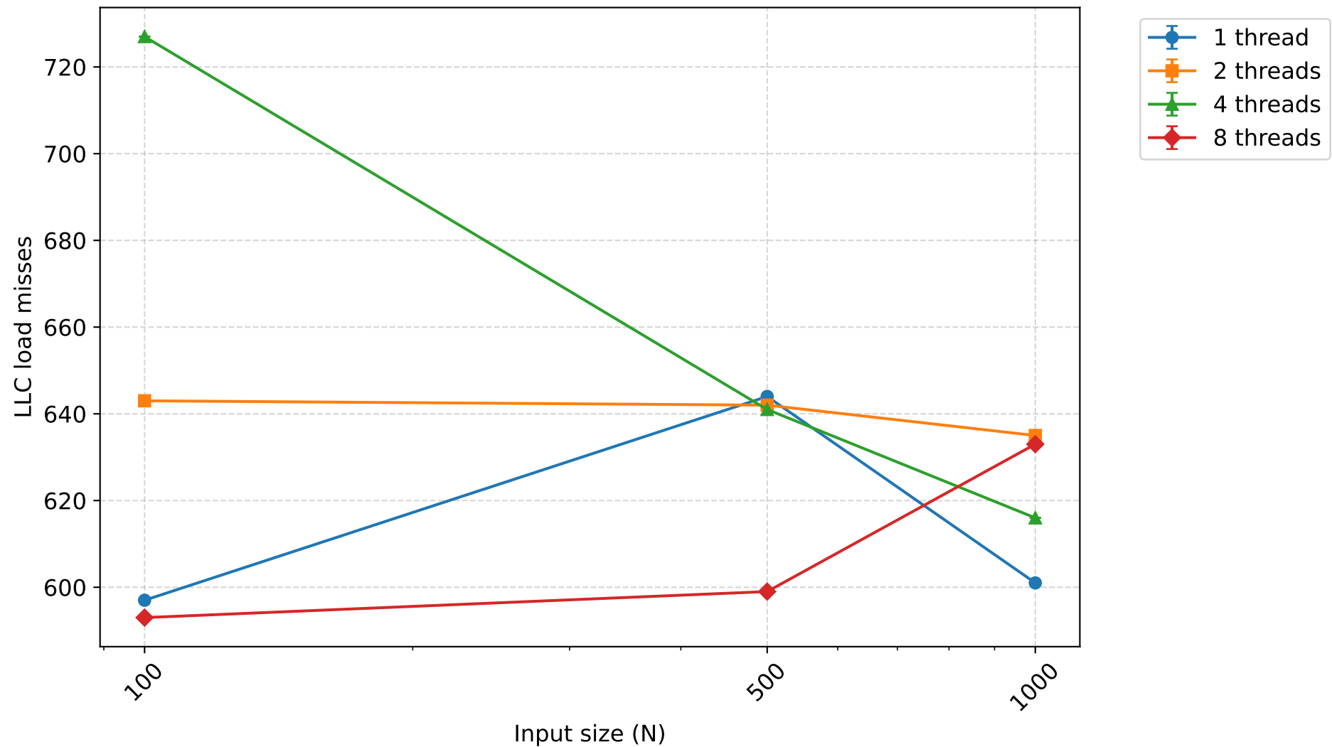
LLC load misses - combSORT (mean \pm 95% CI)
