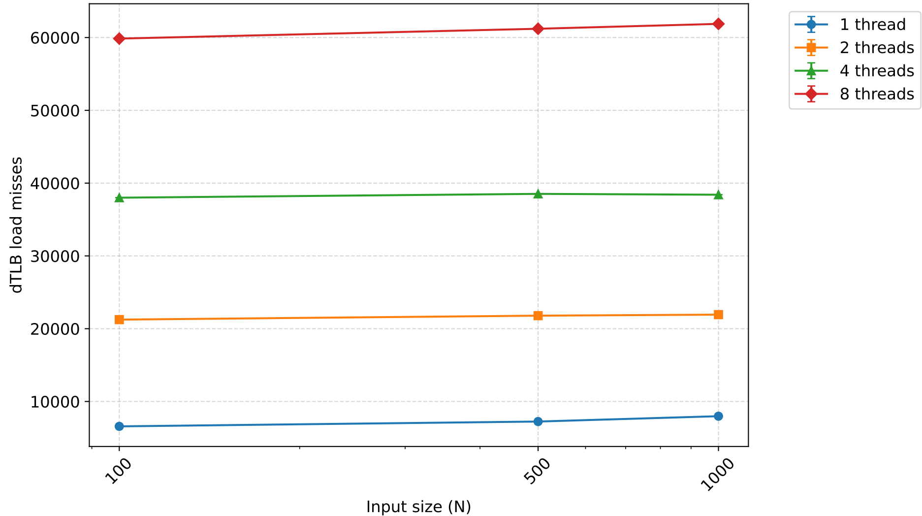
dTLB load misses - counting sort (mean \pm 95% CI)
