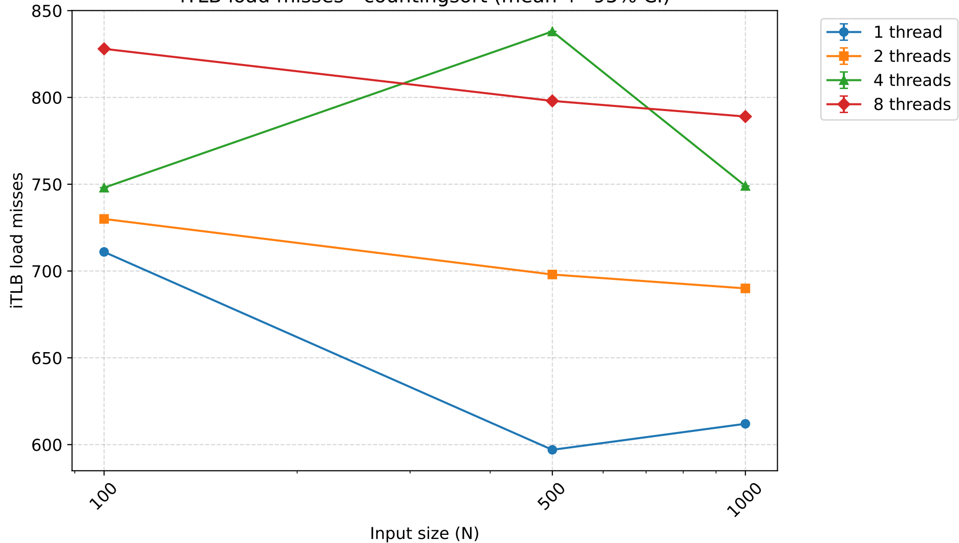
iTLB load misses - counting sort (mean \pm 95% CI)
