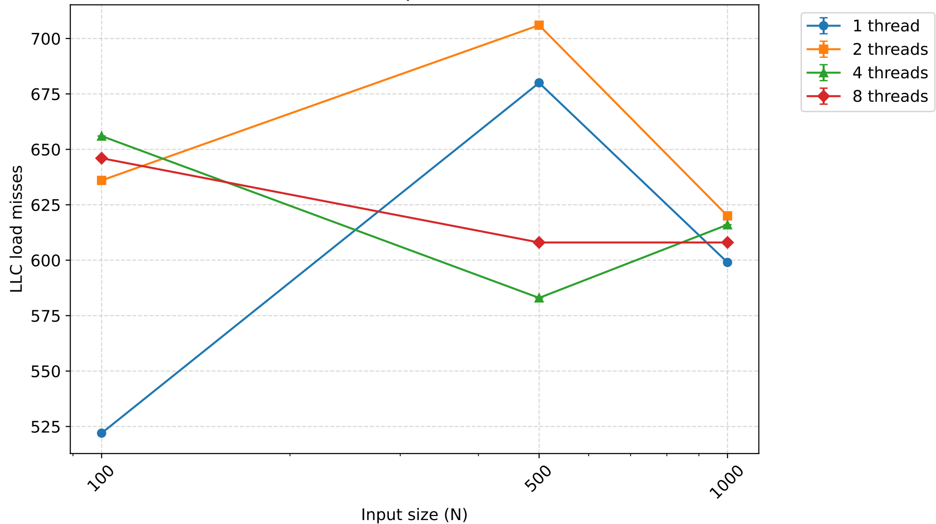
LLC load misses - heapsort (mean \pm 95% CI)
